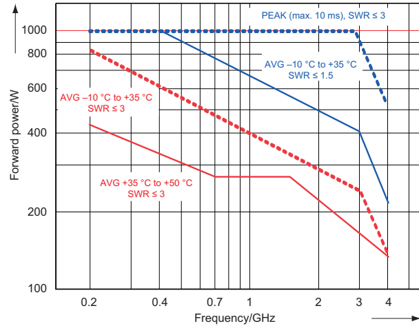
Power-handling capacity.
