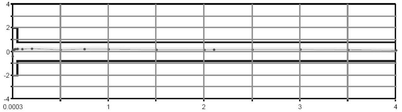
Output power accuracy in dB versus frequency in GHz of R&S®ZVB4
