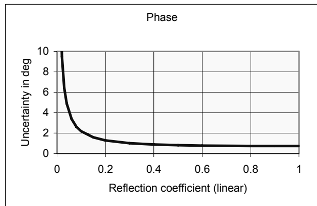
Typical accuracy of reflection magnitude and reflection phase measurements of R&S ® ZVB4 in the frequency range from 300 kHz to 4 GHz, of R&S ® ZVB8 in the frequency range from 300 kHz to 8 GHz, and of R&S ® ZVB20 in the frequency range from 50 MHz to 20 GHz
