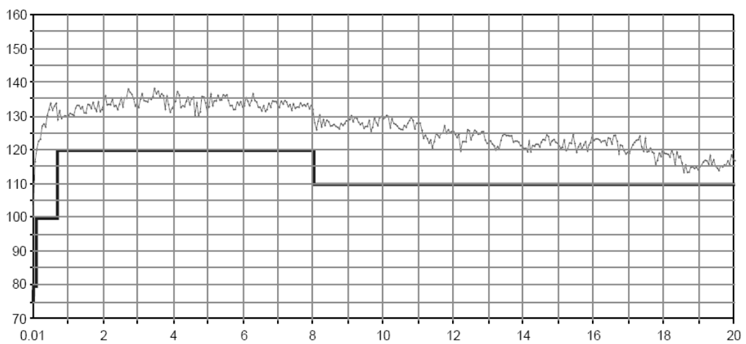
Dynamic range in dB versus frequency in GHz range of R&S®ZVB20
