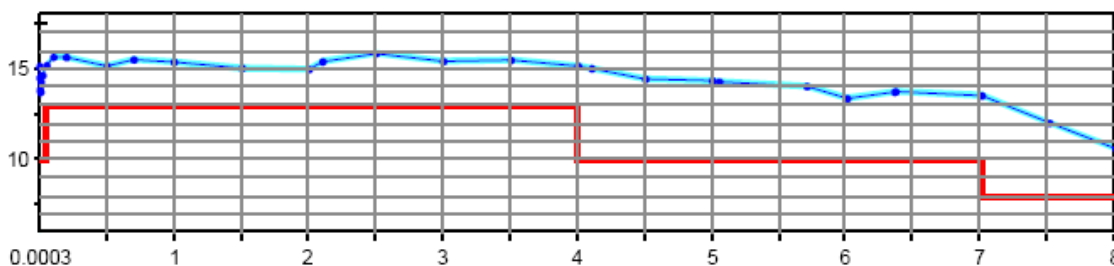
Maximum output power in dBm versus frequency in GHz of the R&S®ZVA8.
