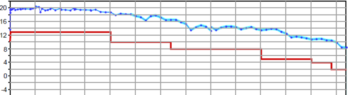
Maximum output power in dBm versus frequency in GHz of the R&S®ZVA67.
