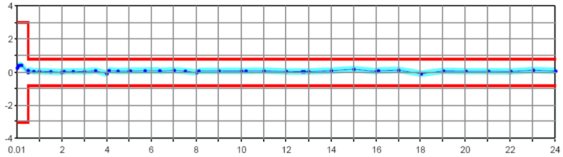
Output power accuracy in dB versus frequency in GHz of the R&S®ZVA24.
