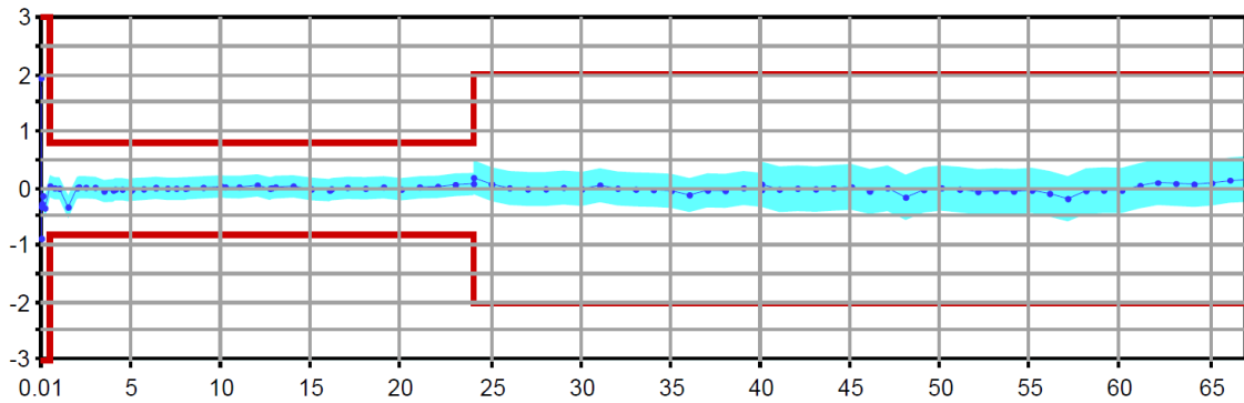
Output power accuracy in dB versus frequency in GHz of the R&amp;S®ZVA67.
