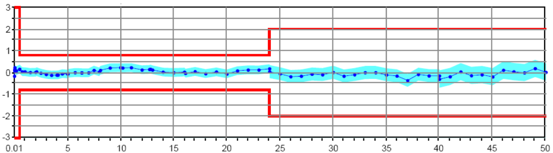
Output power accuracy in dB versus frequency in GHz of the R&S®ZVA50.
