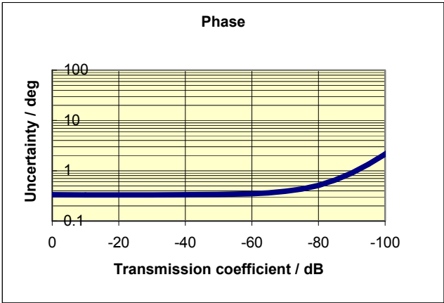
Typical accuracy of transmission magnitude and transmission phase measurements of the R&S®ZVA8 in the frequency range 50 MHz to 8 GHz.
