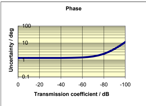
Typical accuracy of transmission magnitude and transmission phase measurements of the R&S®ZVA40 in the frequency range 24 GHz to 40 GHz.
