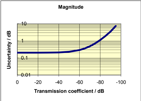
Typical accuracy of transmission magnitude and transmission phase measurements of the R&S®ZVA67 in the frequency range 50 GHz to 67 GHz.
