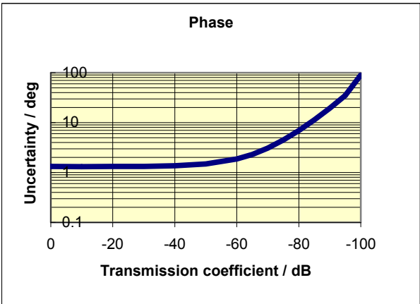
Typical accuracy of transmission magnitude and transmission phase measurements of the R&S®ZVA67 in the frequency range 50 GHz to 67 GHz.
