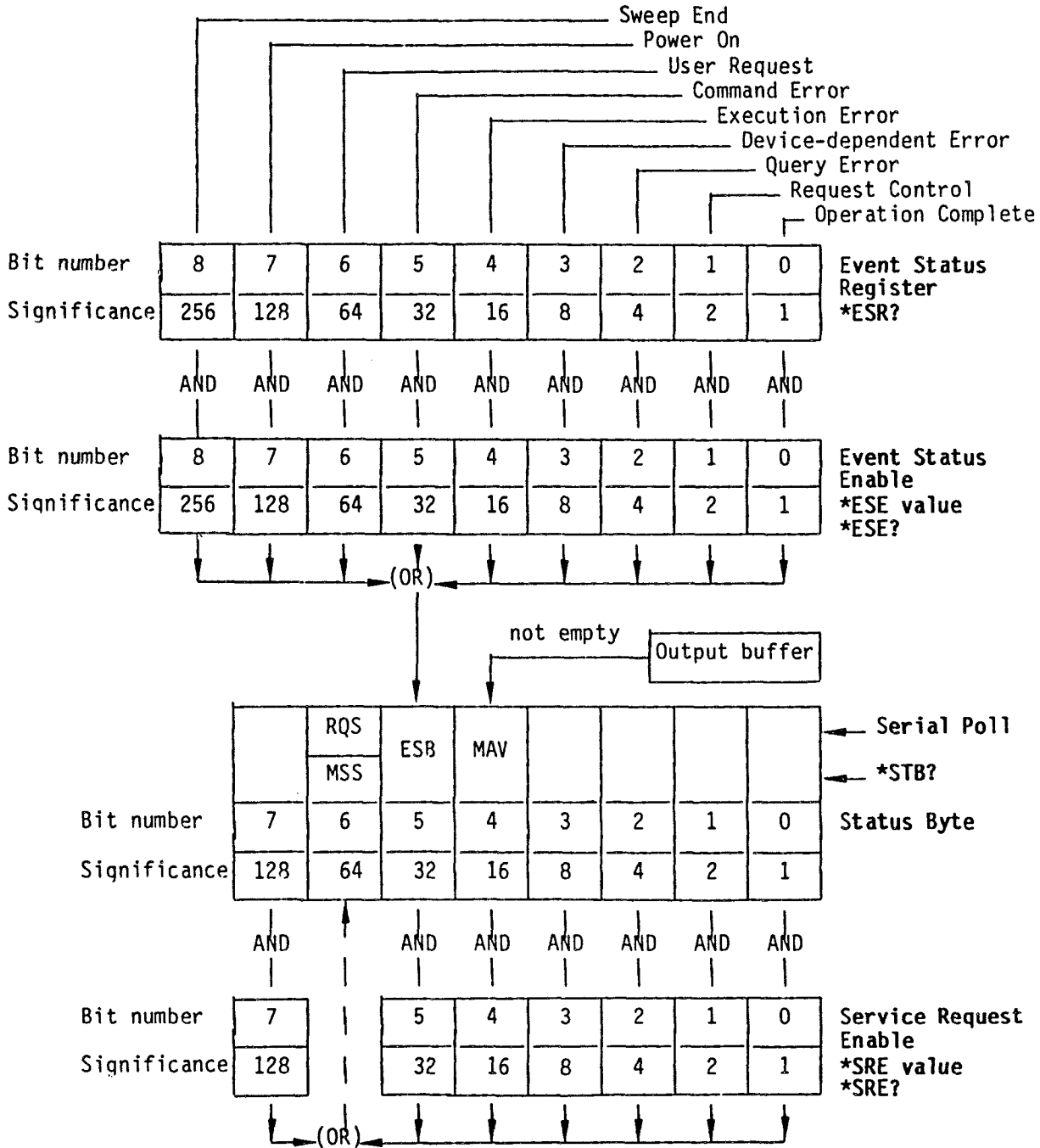
Fig. 2-16 Status registers
