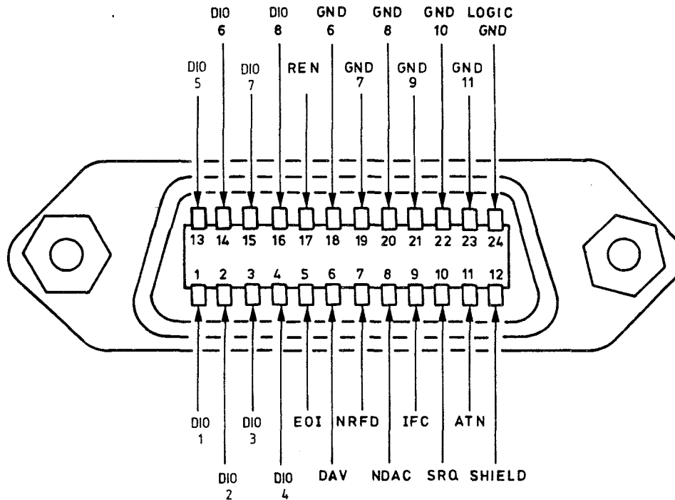
Fig. 2-13 Pin assignments
