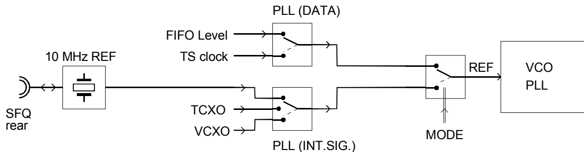
Fig. 2.2.4-25 Reference clock of CS+ coder
