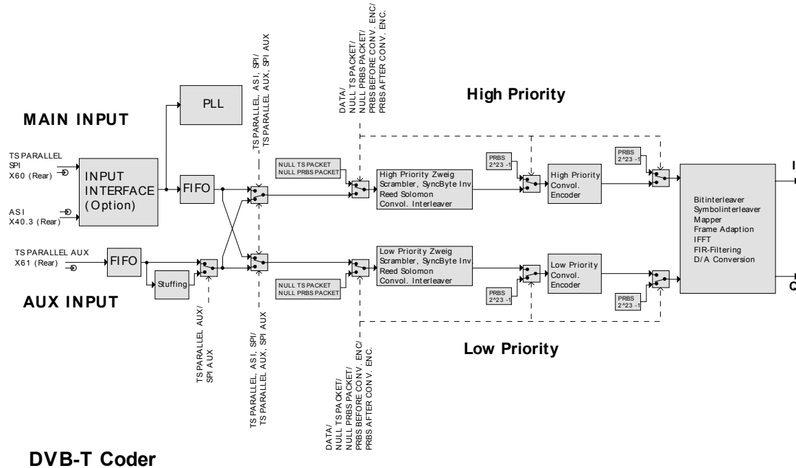
Fig.: 2.2.4-46 Block diagram with input interface and hierarchical coding options
