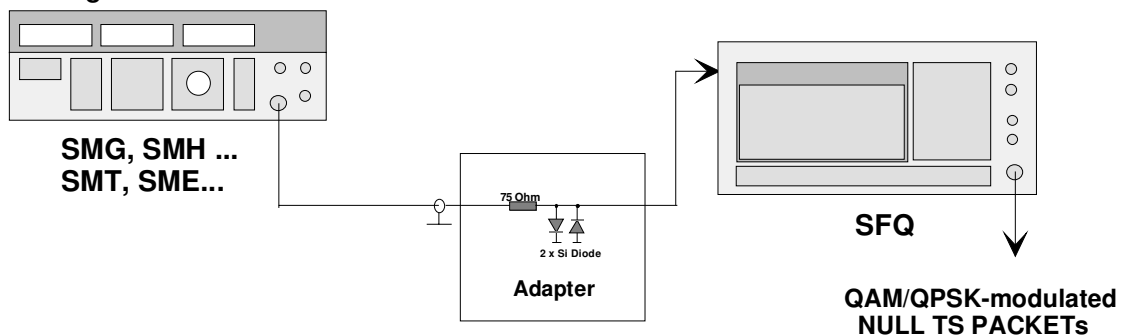
Fig. 1.3-2 Circuit diagram
