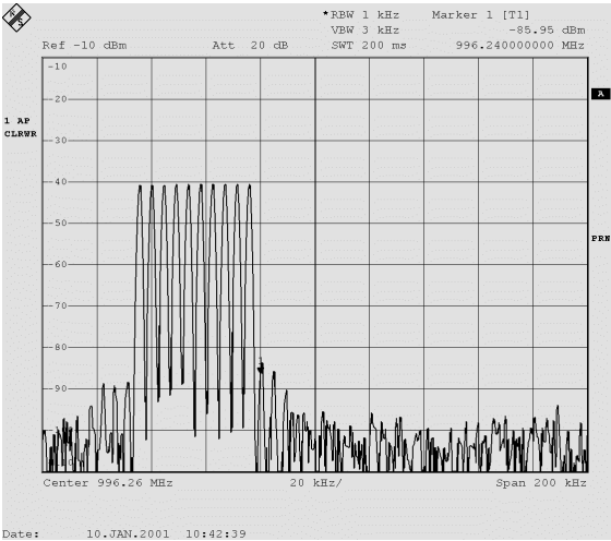
Fig.: 2.2.4-57 EQUAL CW CARRIERS
