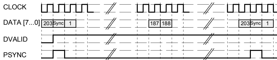
Fig.: 2.2.4-94 Transmission format with packets of 204 bytes (188 bytes of payload and 16 additional bytes)
