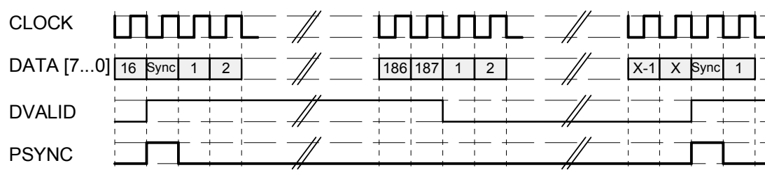
Fig.: 2.2.4-95 Partial TS with a packet length of 188 bytes and x dummy bytes between TS packets
