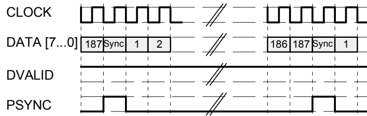
Fig.: 2.2.4-92 Transmission format with packets of 188 bytes
