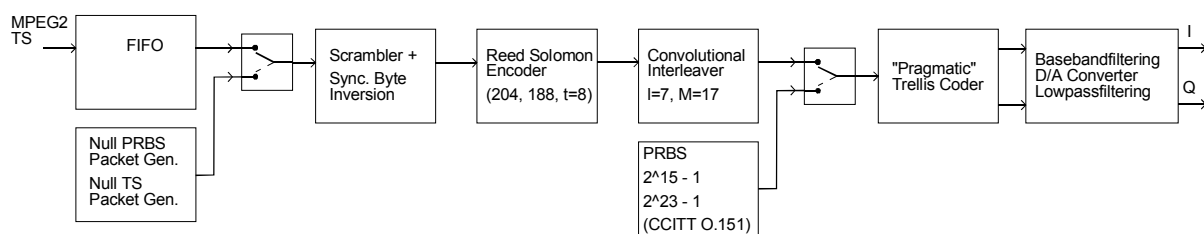
Fig. 2.2.4-2 DVB-S 8PSK and DVB-S 16QAM channel coding
