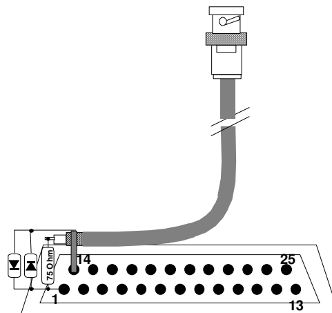
View of solder contacts
