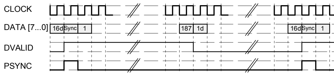
Fig.: 2.2.4-93 Transmission format with packets of 204 bytes (188 bytes of payload and 16 dummy bytes)
