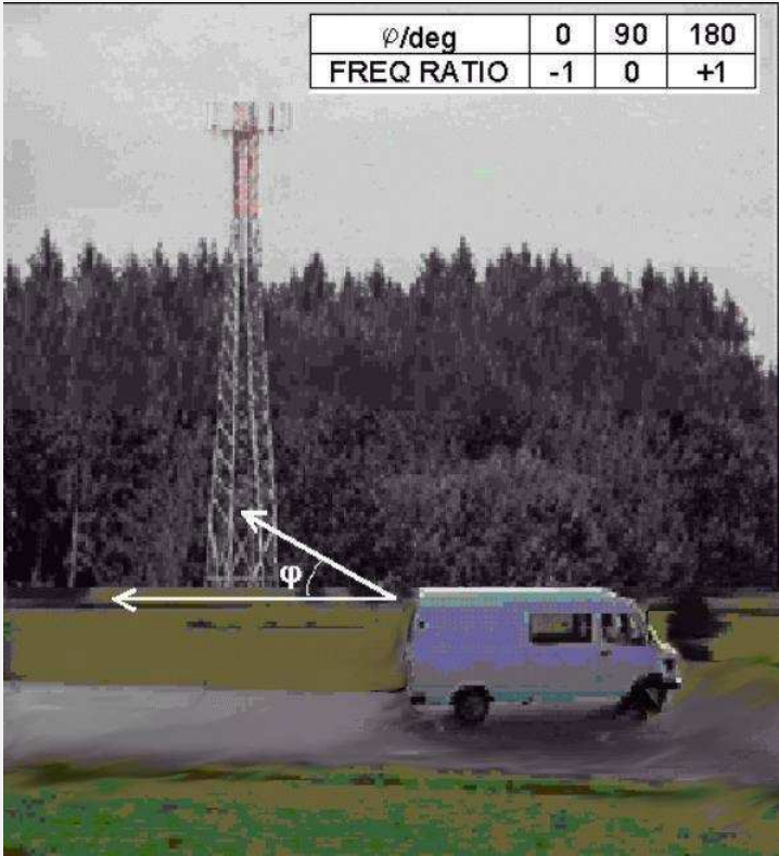
Fig.: 2.2.8-13 Doppler frequency shift with moving receiver
