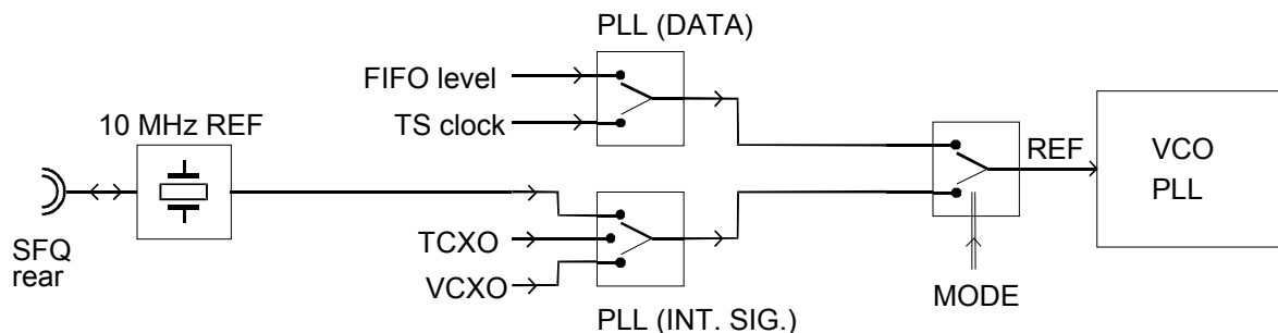
Fig. 2.2.4-13 Reference clock for CS+ coder
