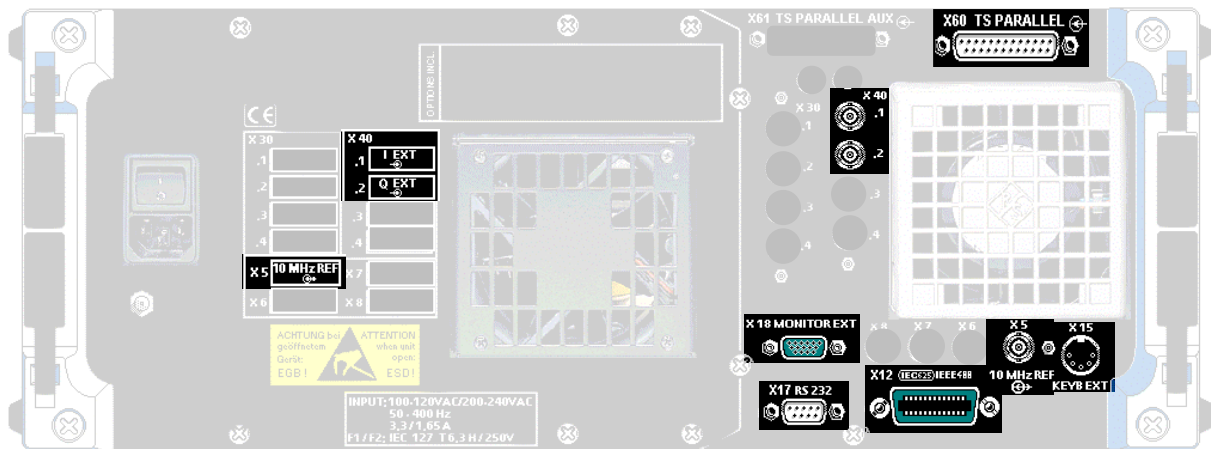
Fig. 1-5 Standard Pin Assignments
