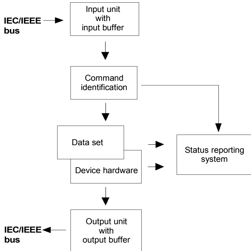
Fig. 3.7-1 Device model with remote control via IEC/IEEE bus
