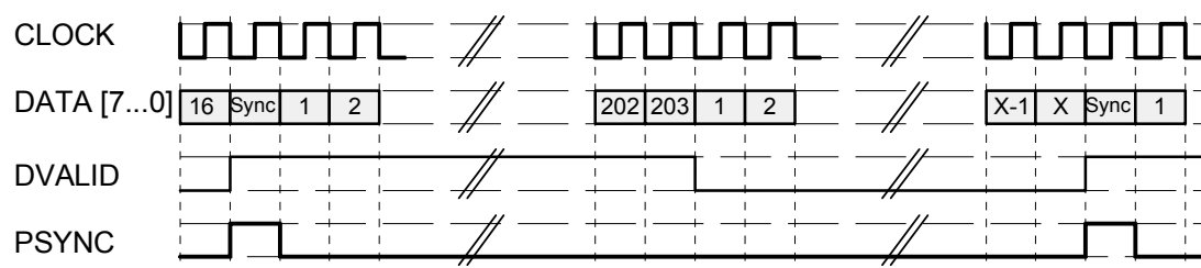
Fig.: 2.2.4-96 Partial TS with a packet length of 204 bytes and x dummy bytes between TS packets
