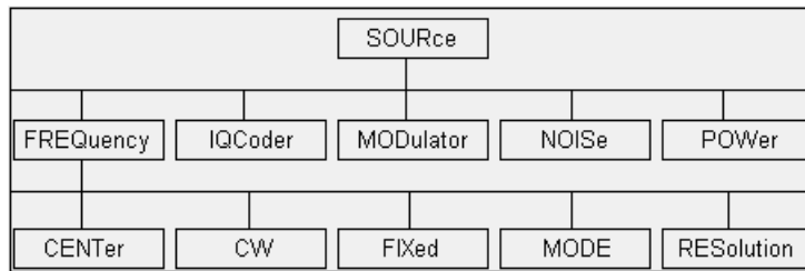
Fig. 3-1 Tree structure of SCPI command system, SOURce being shown as an example
