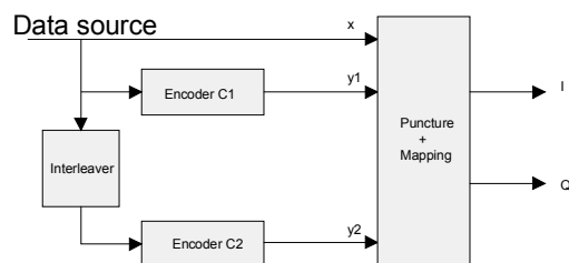
Fig. 2.2.4-15 Structure of turbo encoder
