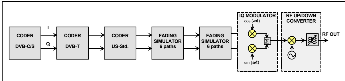
Fig.: 2.2.8-1 Fading simulator in SFQ
