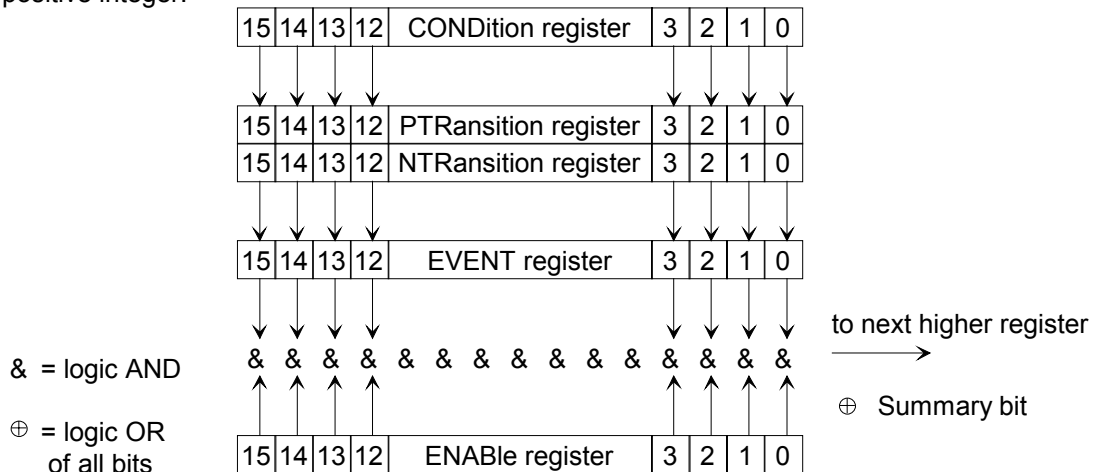
Fig. 3.8-1 Status register model
