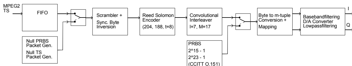
Fig.: 2.2.4-26 DVB-C QAM channel coding
