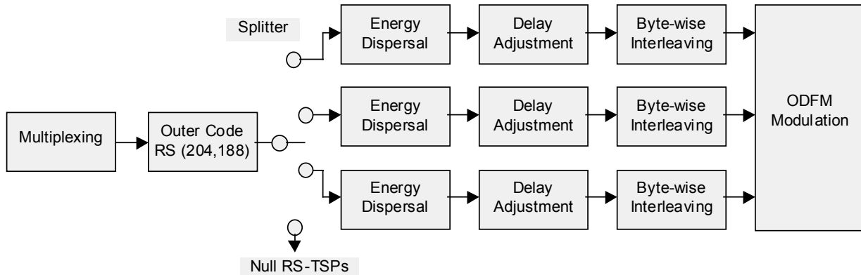
Fig. 2.2.4-77 Channel coding block diagram
