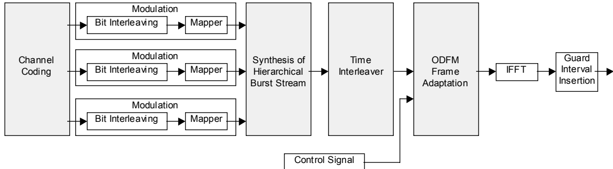
Fig. 2.2.4-78 Modulation block diagram
