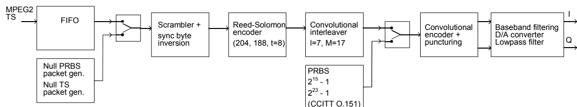
Fig. 2.2.4-1 DVB-S QPSK channel coding
