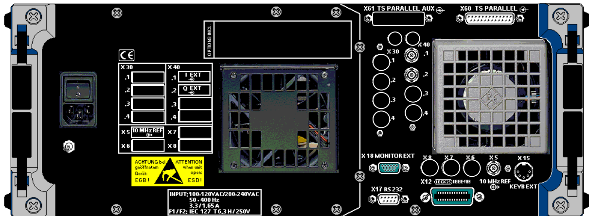
Fig. 1-4 Rear View
