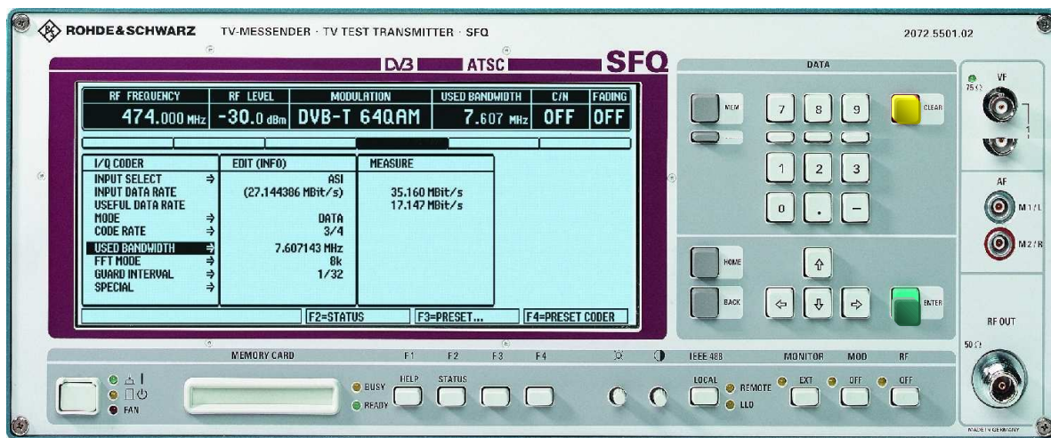
Fig. 2-1 Front panel
