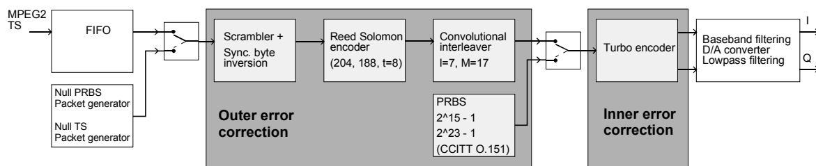
Fig. 2.2.4-14 Channel coding in Turbo mode
