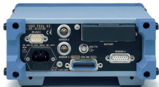
The battery, the R&S® NAP sensor connector and two R&S® NRT sensor connectors are accessible on the rear panel
