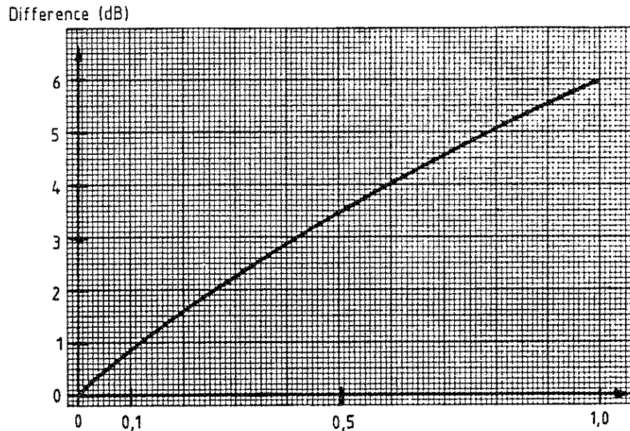
Fig. 2-17 Increase in peak-value indication as against average-value indication with amplitude modulation
