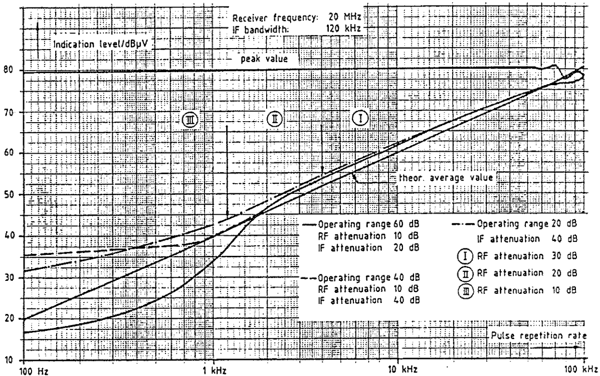
Fig. 2-24.1 Peak- and average-value indication as a function of the pulse repetition rate
