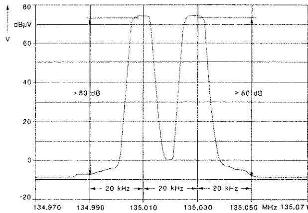
Two-tone measurement on Test Receiver ESVP
