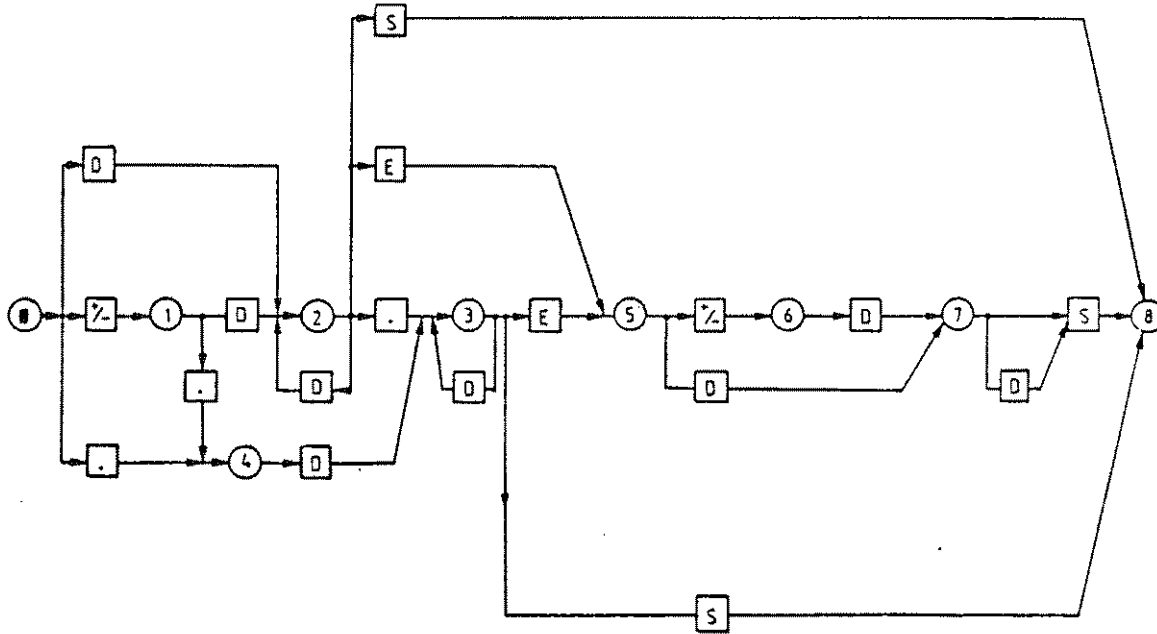
Fig. 2-13 IEC-bus syntax diagram (Only to illustrate the processing by the ESVP. It shows, among other things, that the ESVP can also process numbers in exponential form.)
