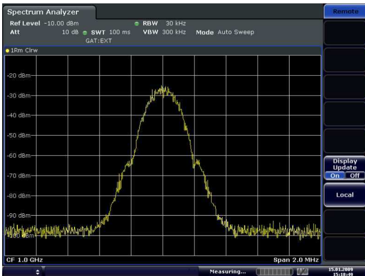
Figure 6-16: TDMA signal with GATE ON
