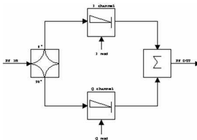
Figure 8-9: I/Q modulation
