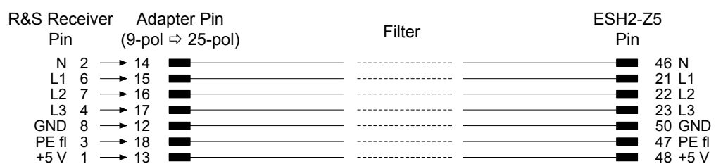
Figure 5-5: Connection from R&S ESR to R&S ESH2-Z5
