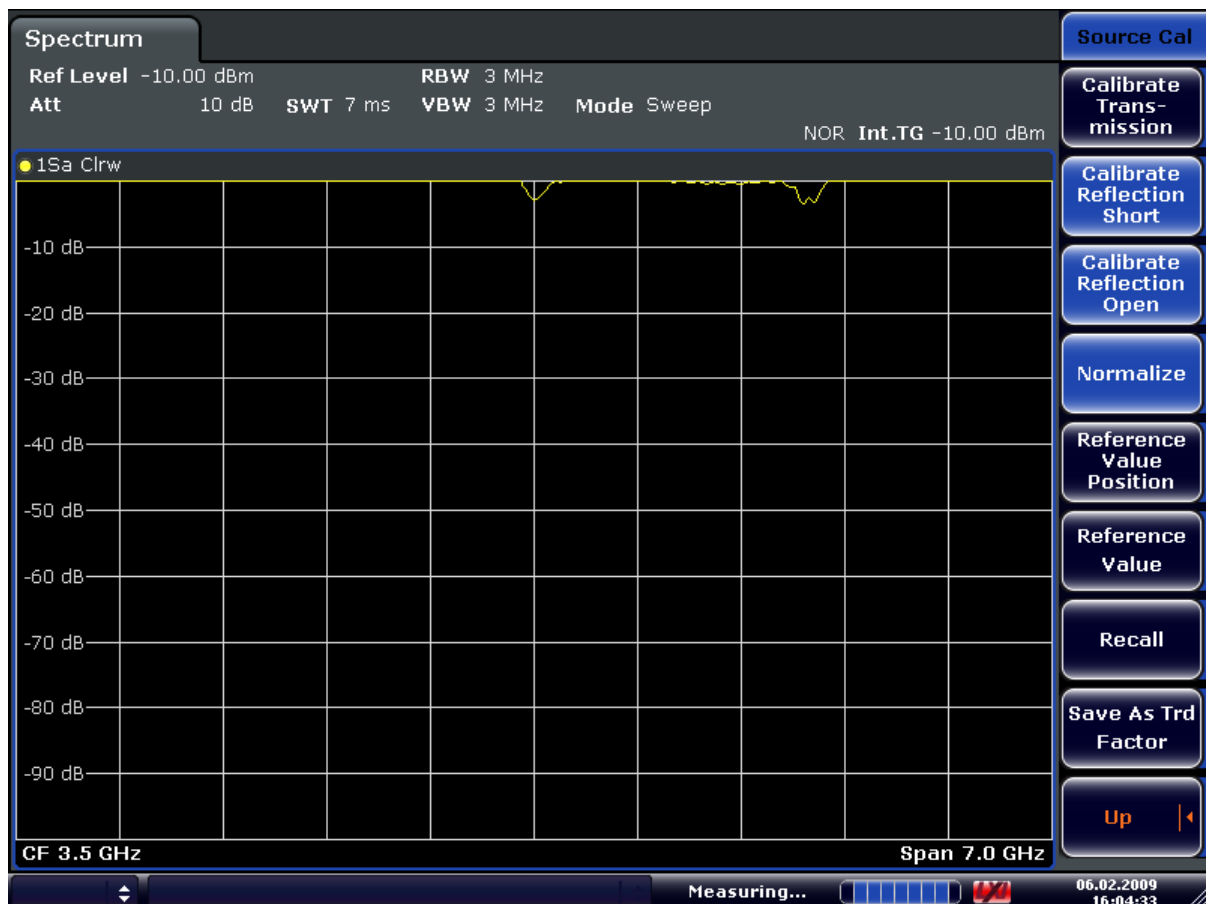
Figure 8-5: Normalized display
