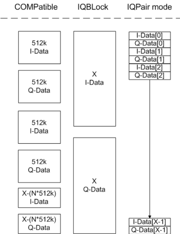
Figure 11-5: IQ data formats
