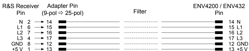
Figure 5-8: Connection from R&amp;S ESR to R&amp;S ENV4200 or R&amp;S ENV432
