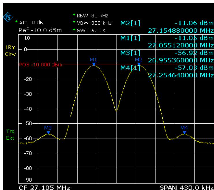
Figure 6-21: Trace example
