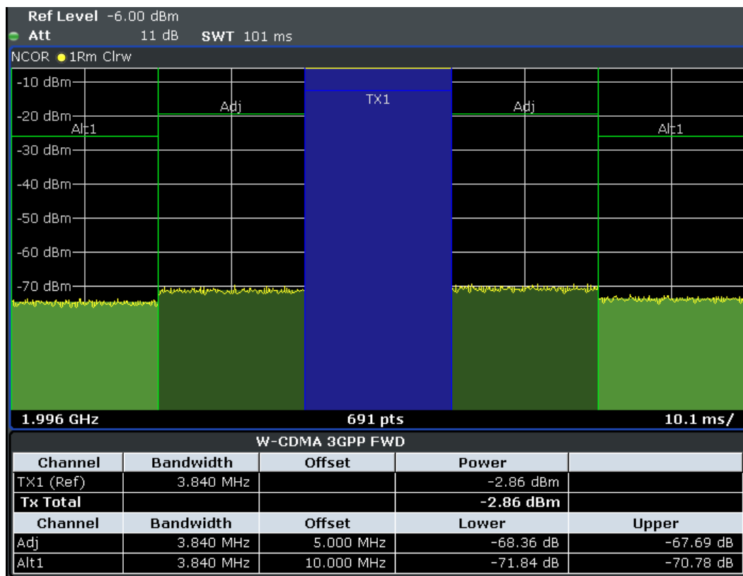
Figure 6-34: Measuring the adjacent channel power of a W-CDMA signal with the fast ACLR mode
