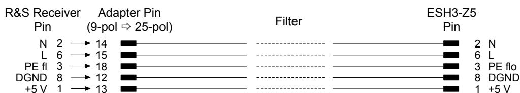
Figure 5-6: Connection from R&amp;S ESR to R&amp;S ESH3-Z5
