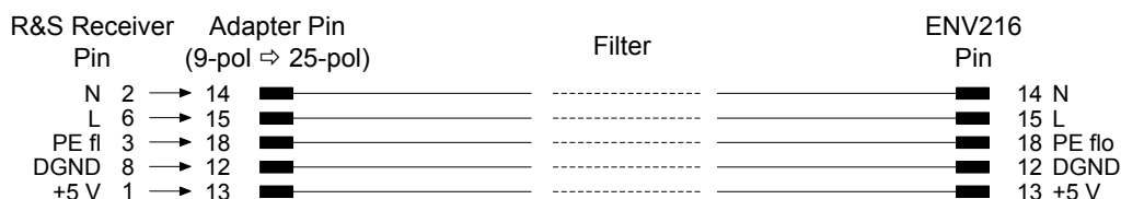
Figure 5-7: Connection from R&amp;S ESR to R&amp;S ESH216
