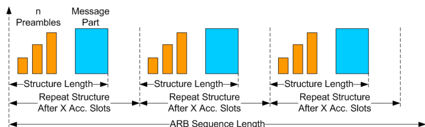
Figure 4-26: "Repeat Structure after ARB sequence length = Off"
