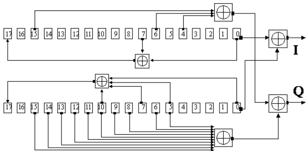
Figure 3-2: Structure of downlink scrambling code generator
