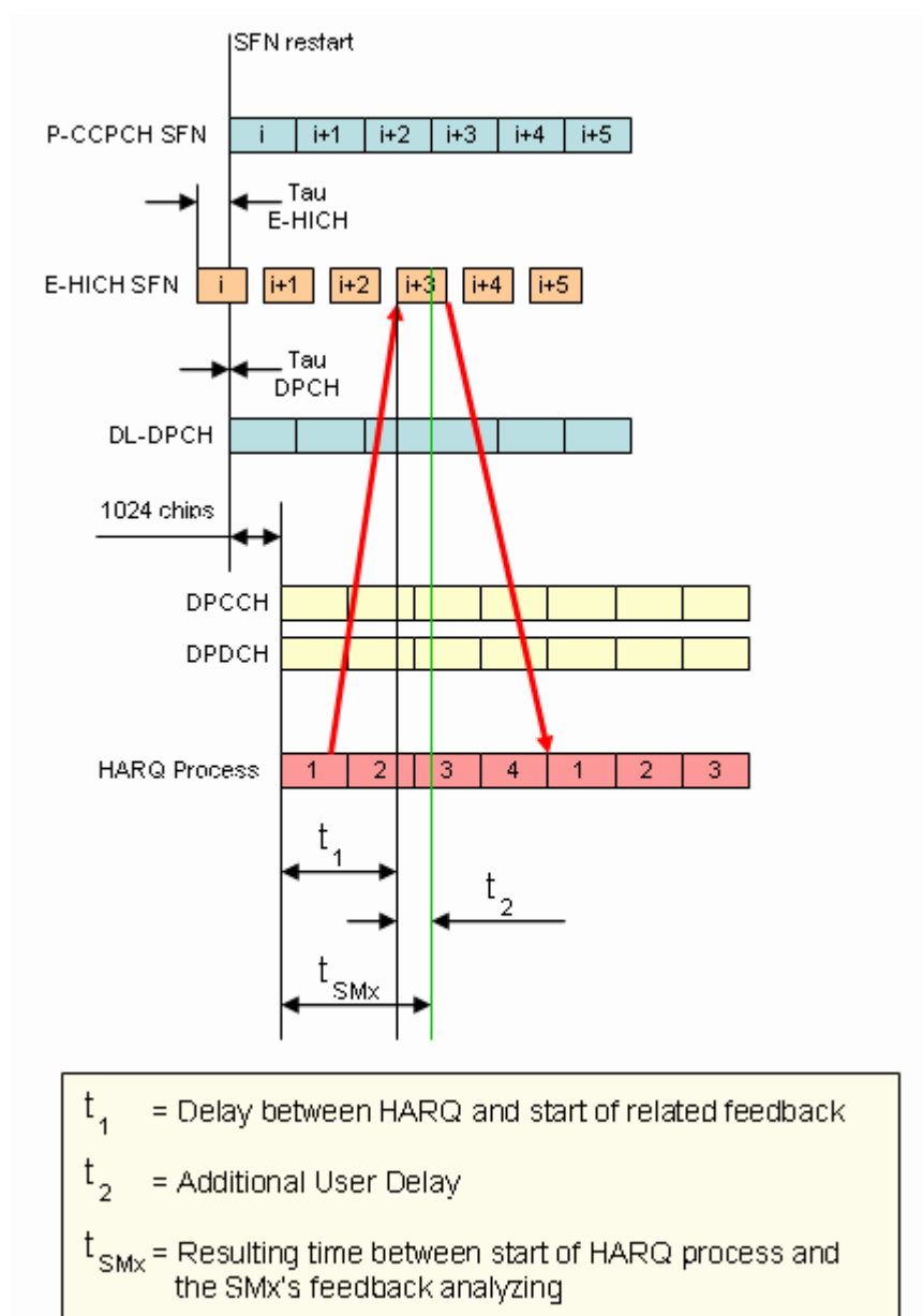
Figure 3-7: Timing diagram for TTI 10ms, \tau_{dpch} = 0 , \tau_{E-HICH} = -7\text{slots}
