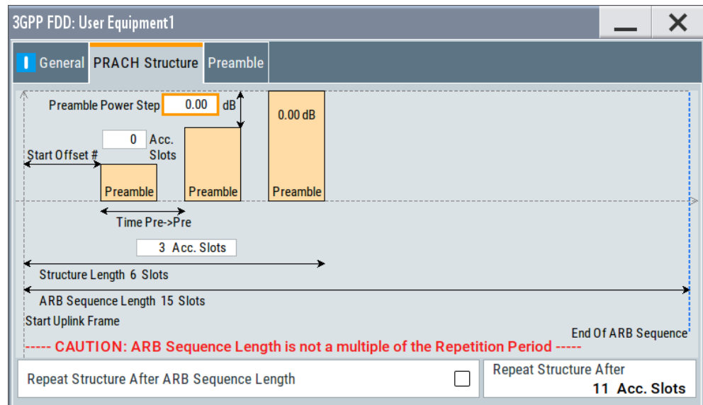
Figure 4-24: PRACH mode Preamble Only
