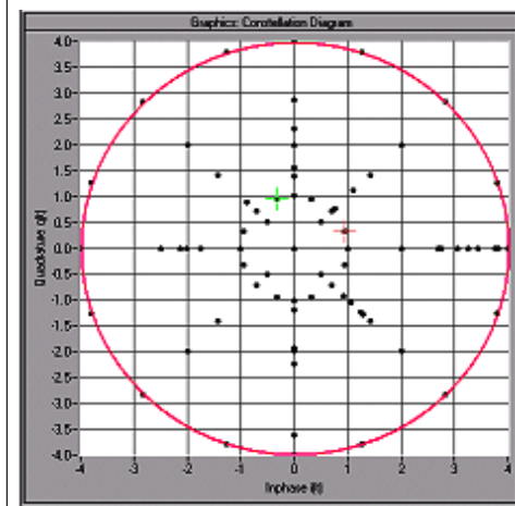
Constellation diagram with clipping level 50 %, vector mode ( |I+Q| )
