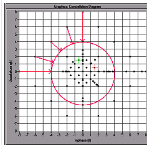
Constellation diagram of the signal without clipping, shows the level mapping for vector mode
