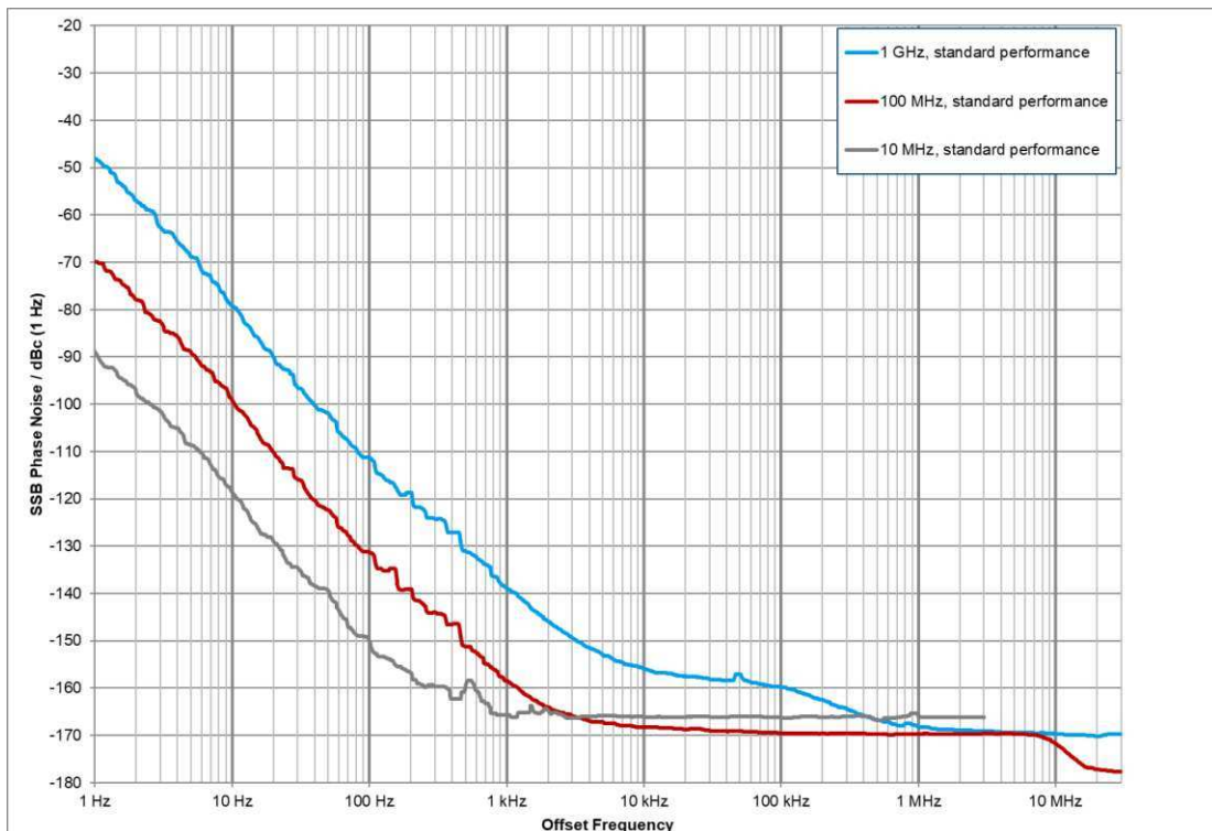
Measured SSB phase noise of reference outputs at f = 10 MHz, 100 MHz and 1 GHz with standard performance ( f = 100 MHz and 1 GHz only available with the R&S ® SMAB-K703 option)
