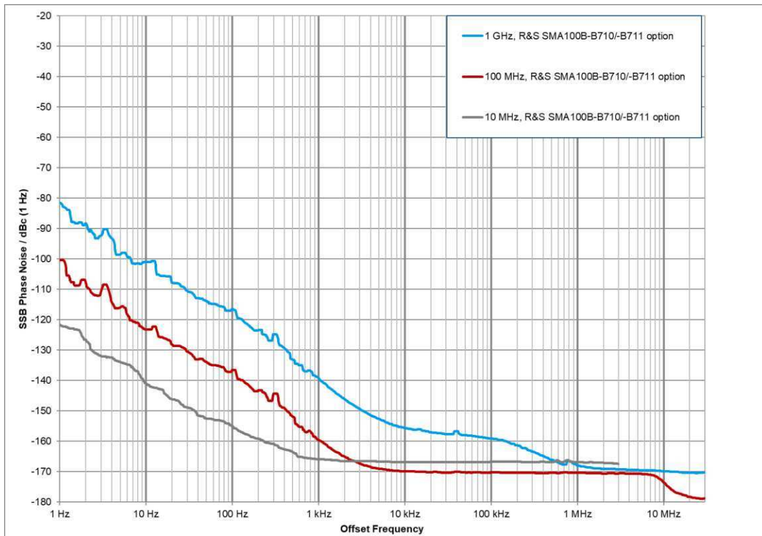
Measured SSB phase noise of reference outputs at f = 10 MHz, 100 MHz and 1 GHz with the R&S ® SMAB-B710(N) and R&S ® SMAB-B711(N) options ( f = 100 MHz and 1 GHz only available with the R&S ® SMAB-K703 option)
