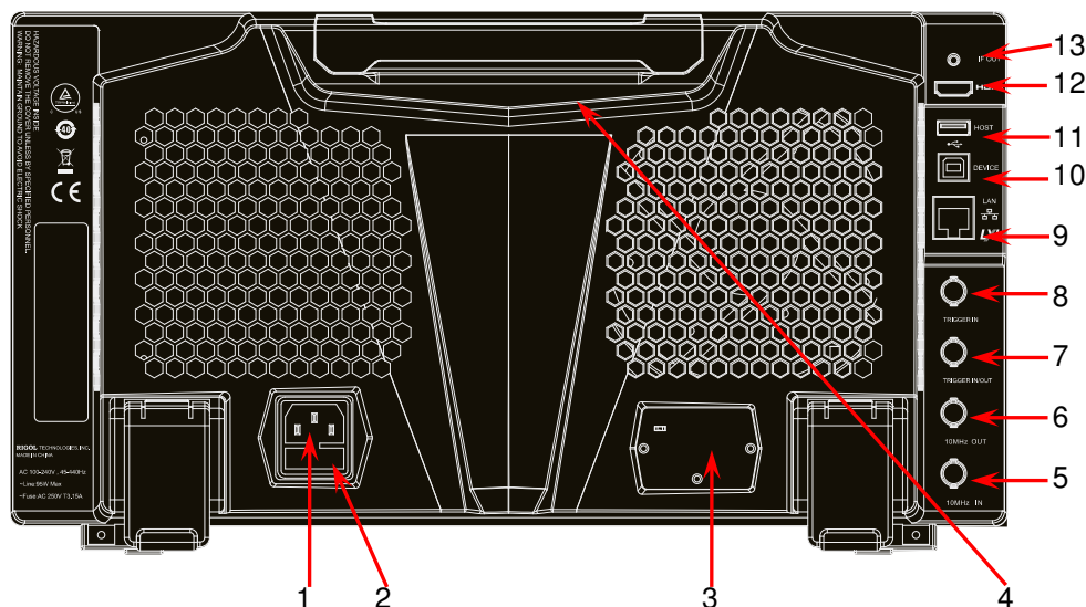
Figure 1-8 Rear Panel
