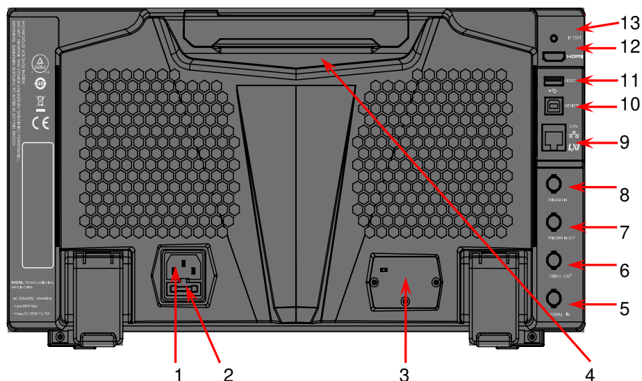
Figure 1-8 Rear Panel
