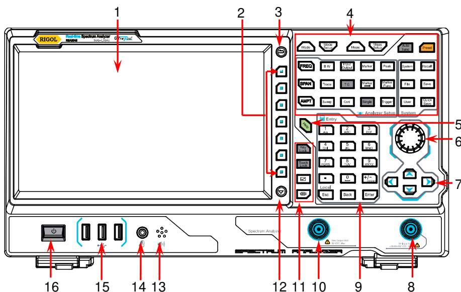
Figure 1-4 Front Panel
