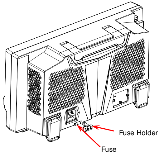
Figure 8 Fuse Replacement
