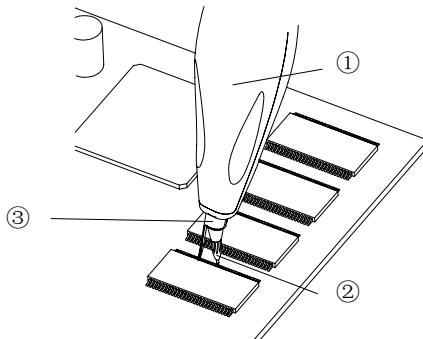
Figure 10 Hand-held Single-ended Probe Head
