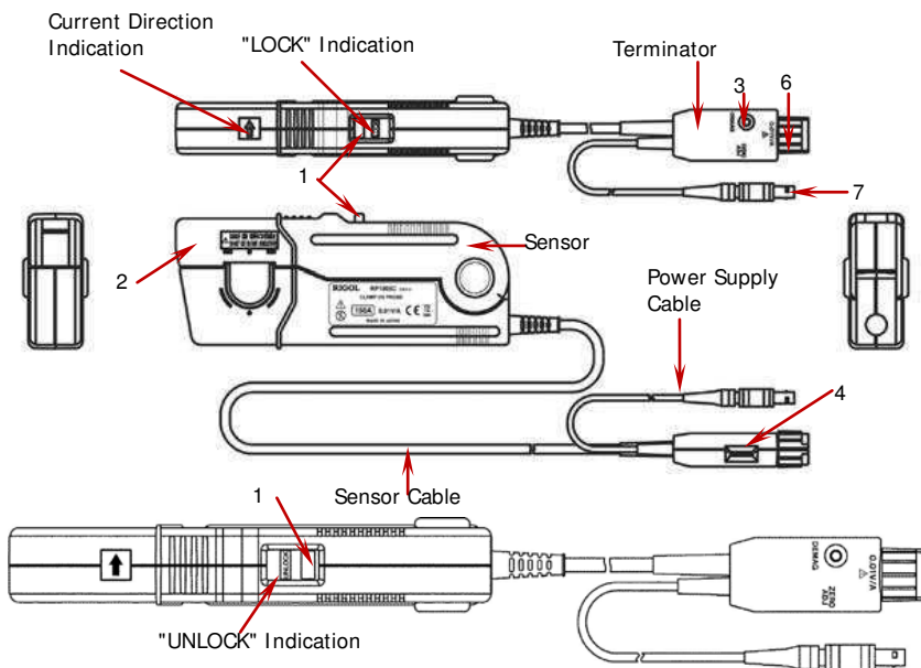
Figure 2 RP1005C Parts
