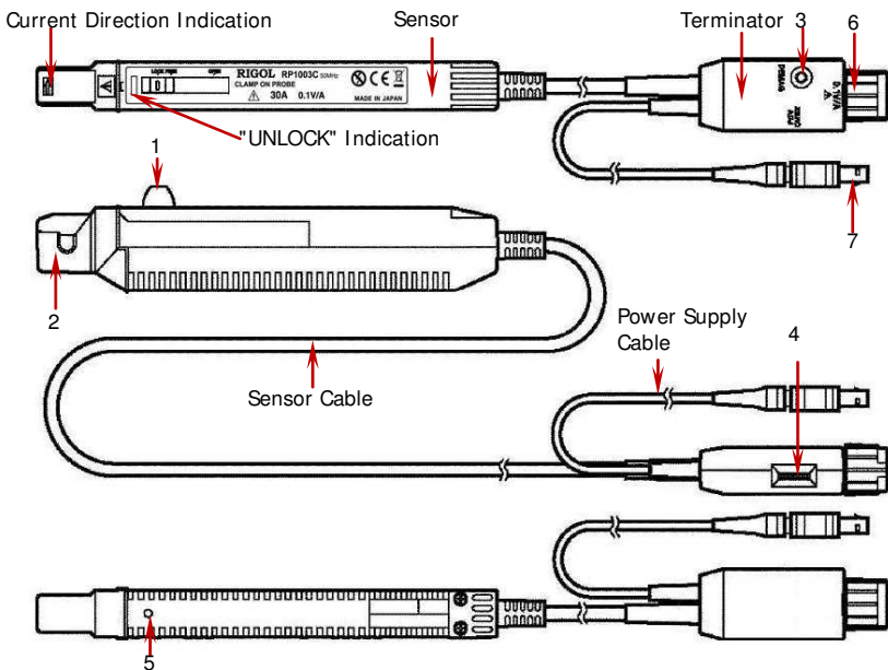
Figure 1 RP1003C/ RP1004C Parts
