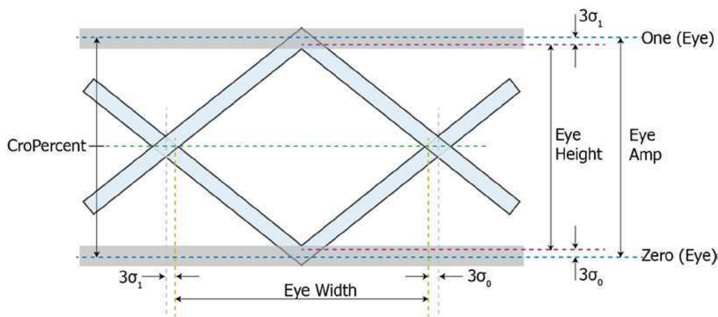
Figure 10-1 Diagram of Eye Measurement Parameters
