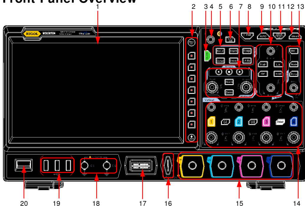
Figure 1-13 Front Panel
