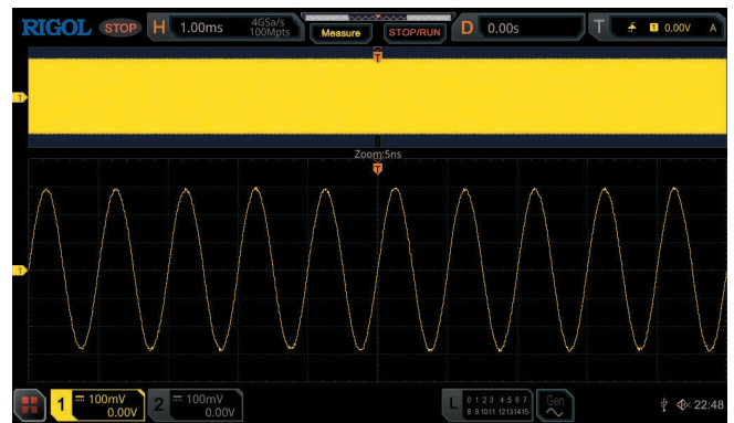
With up to 100 M memory depth, you can capture 12.5 ms of waveforms while maintaining a sample rate of 4 G, without causing the waveforms to be distorted.
