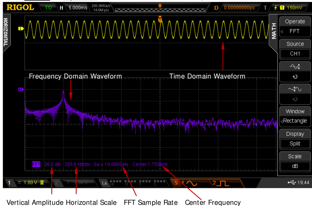
Figure 6-1 FFT Operation
