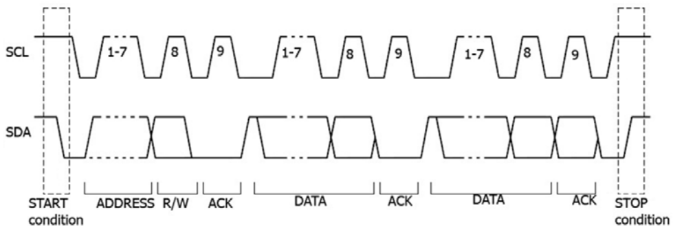
Figure 5-14 I2C Trigger
