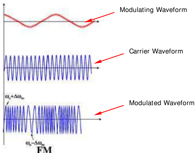
Figure 13-10 Frequency Modulation
