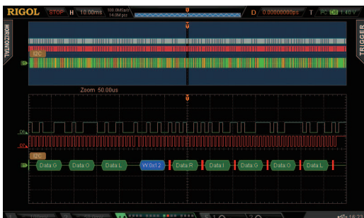
Deeper memory depth for the digital channels, serial bus triggering and decoding on digital channels
