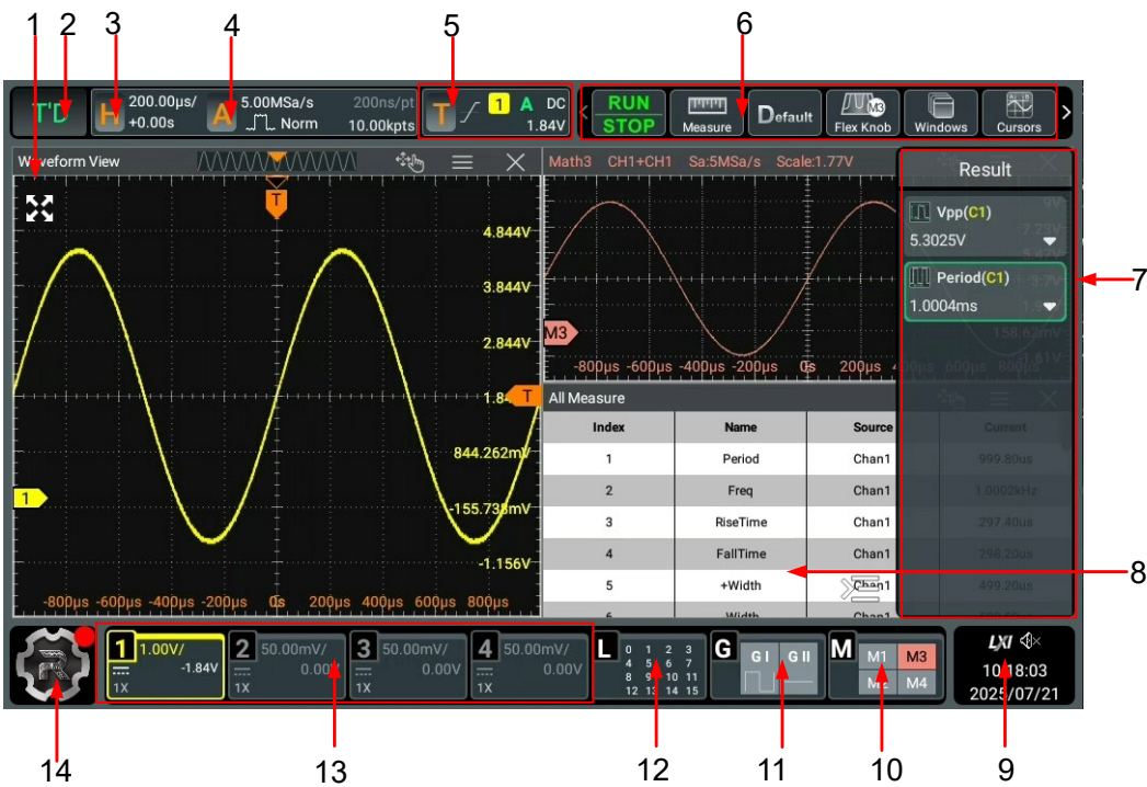
Figure 4.5 User Interface
