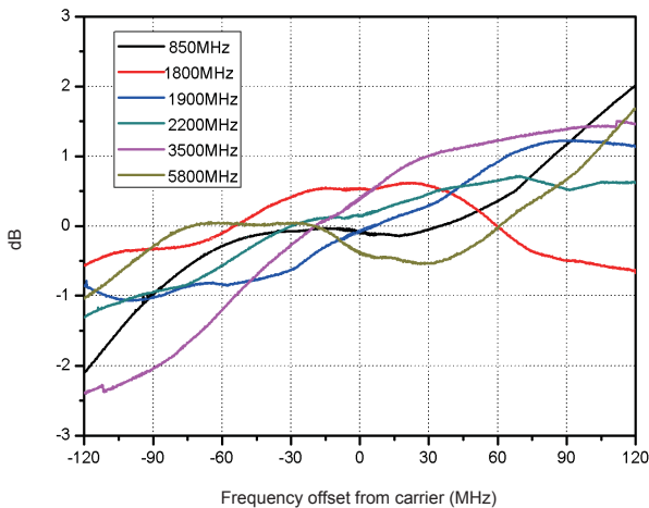
Measured external IQ bandwidth
