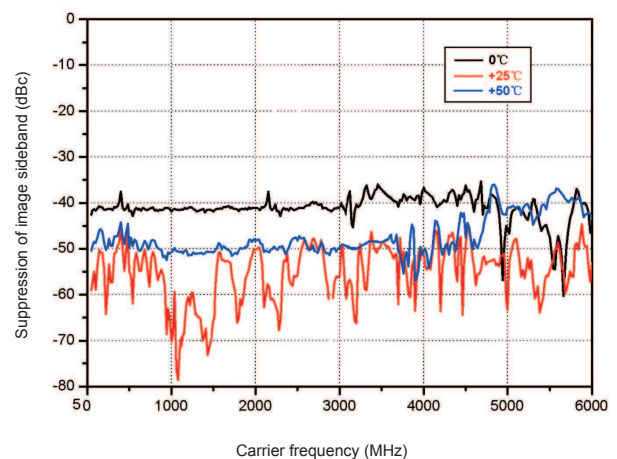
Measured suppression of image sideband
