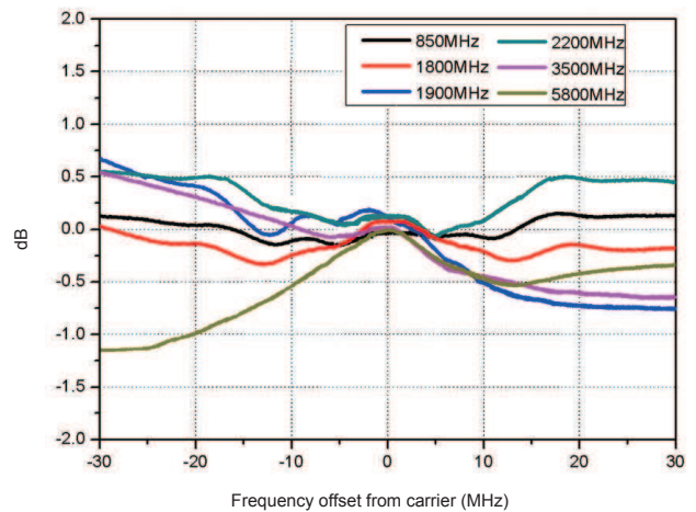
Measured internal IQ bandwidth
