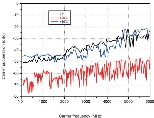
Measured carrier suppression
