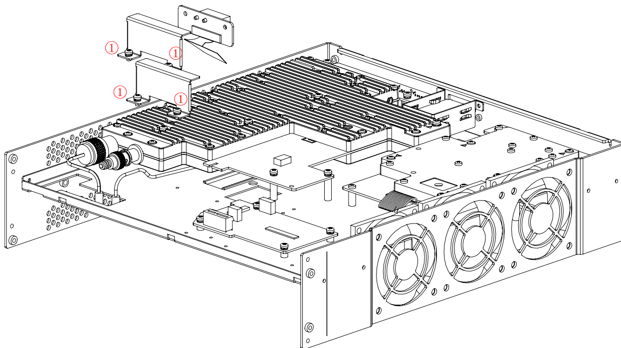
Figure 1-11 Disassemble the PCIe Cables
