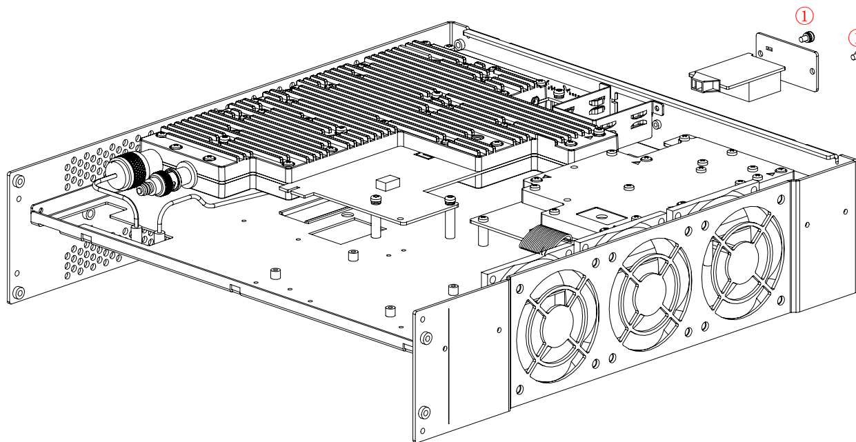
Figure 1-13 Disassemble the OCXO Module
