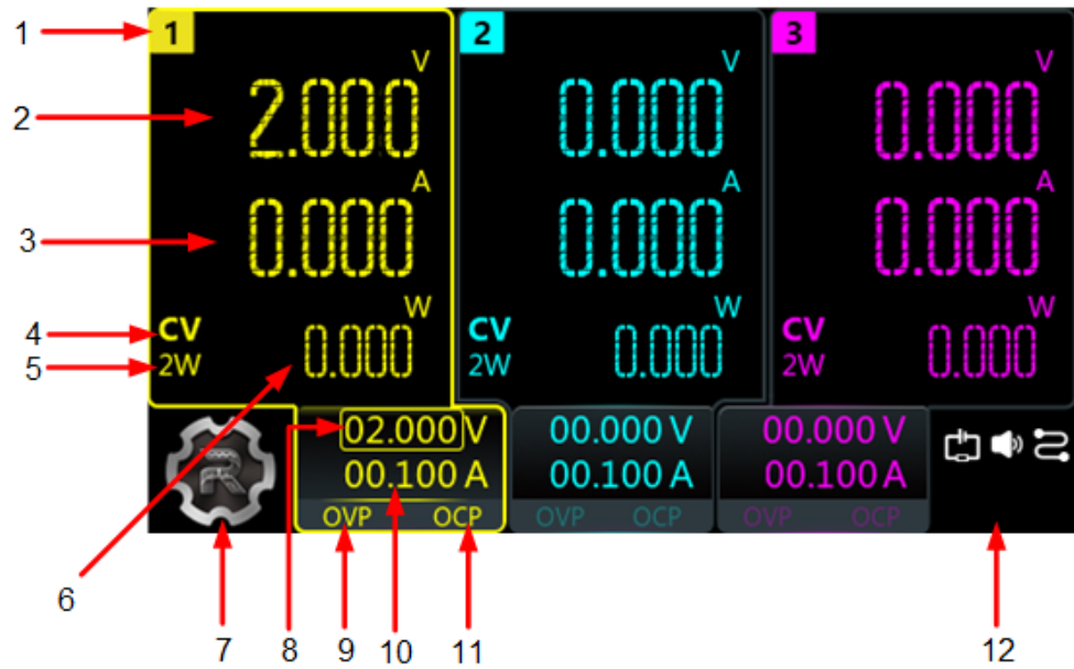
Figure 4.6 User Interface
