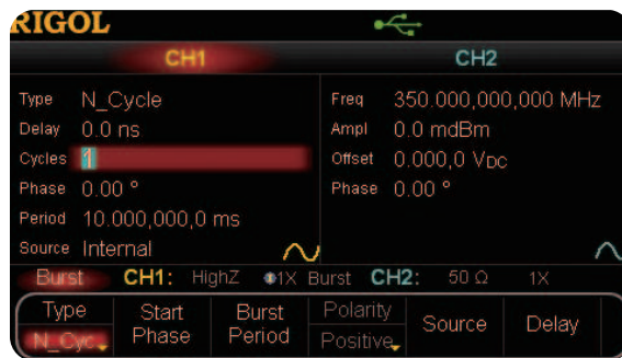
Burst
