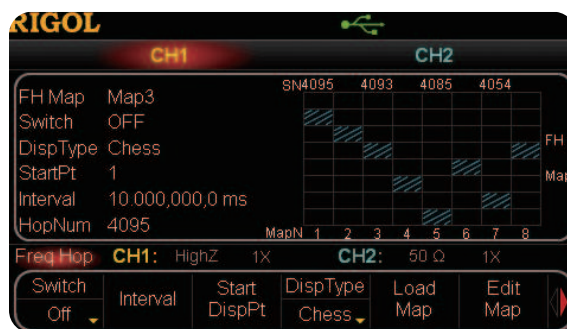
Frequency Hopping
