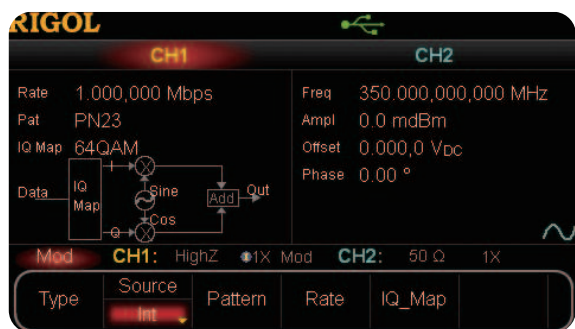
IQ Modulation
