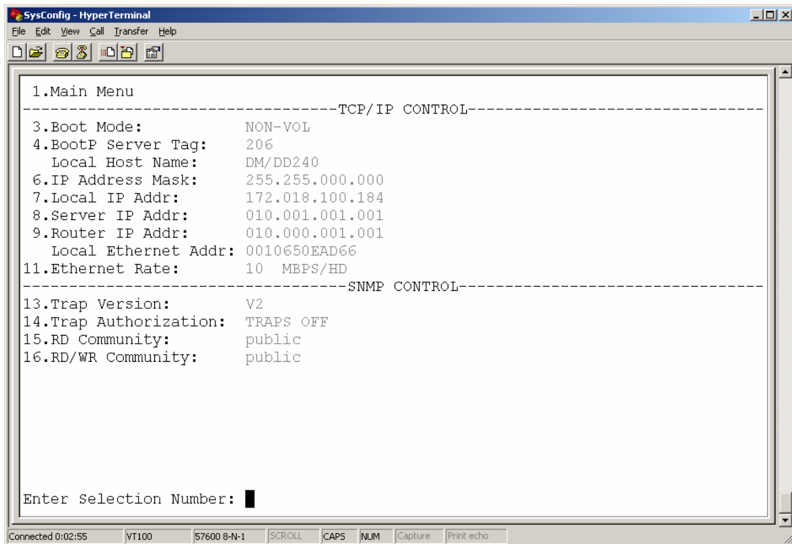
Figure 4-10. TCP/IP/SNMP Control Menu
