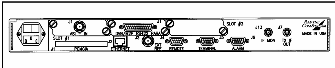
Figure 5-2b. DM240 Rear Panel Connectors (L-Band) with PIIC.
