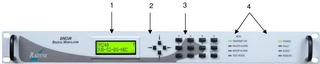
Figure 4-1. DM240 Front Panel
