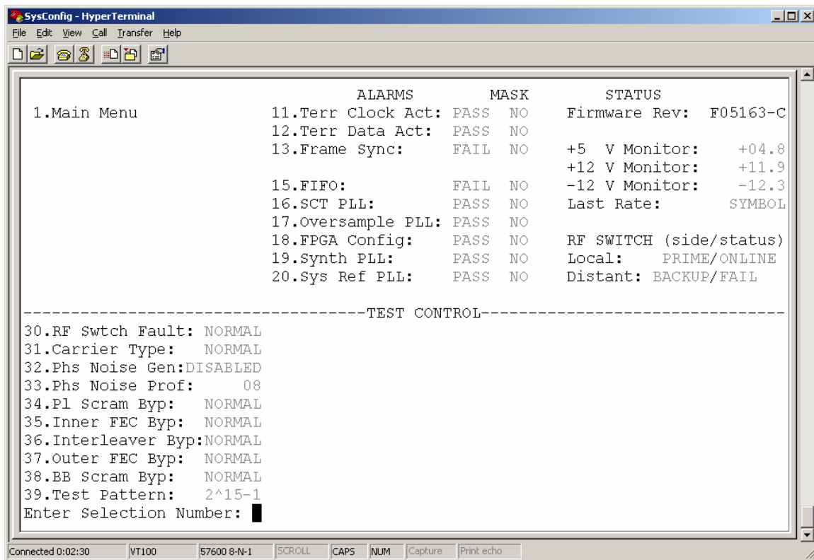
Figure 4-9. Test Control Menu
