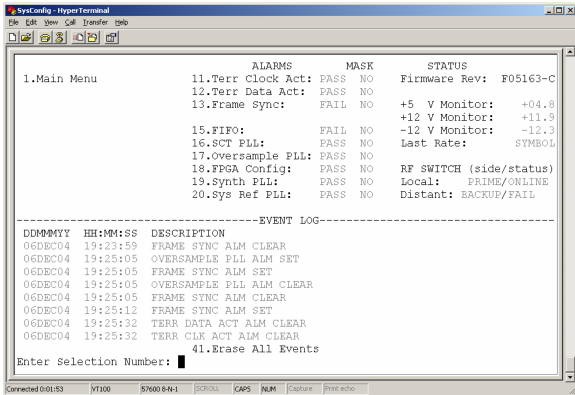
Figure 4-7. Event Log Menu
