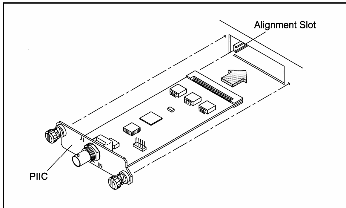
Figure 5-4. Typical PIIC
