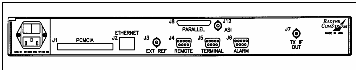
Figure 5-1a. DM240 Rear Panel Connectors (70/140 MHz)
