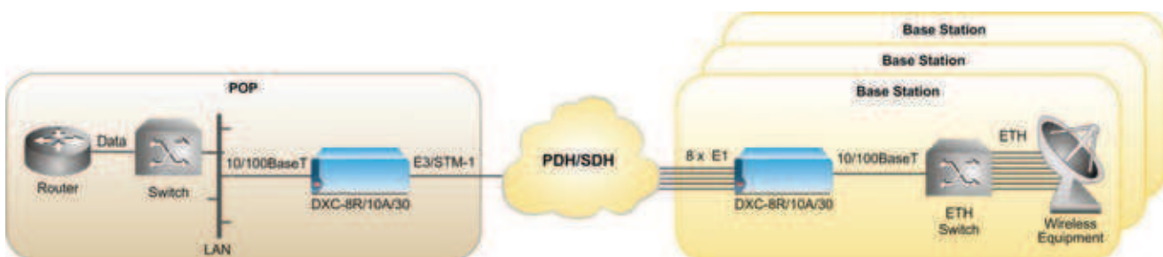
Figure 4. Inverse Multiplexing
