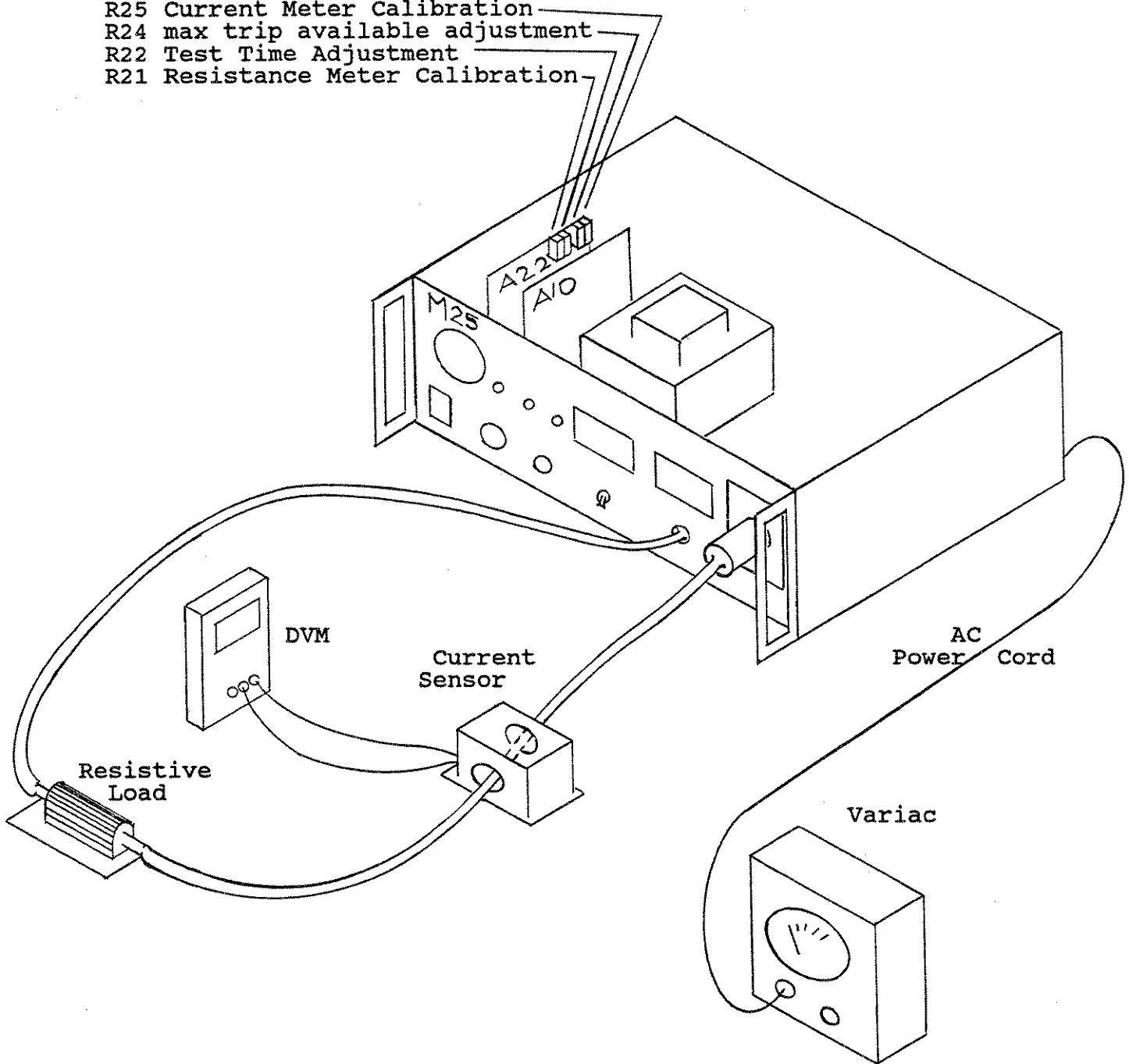
Figure 4-1: Test Set-Up
