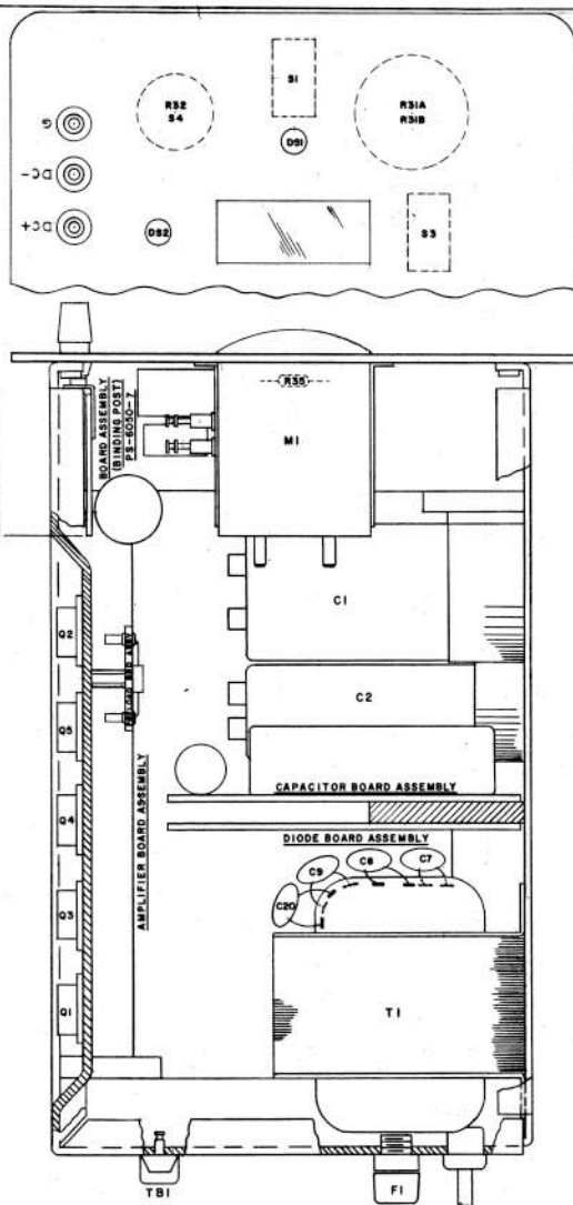
TOP VIEW OF UNIT WITH COVER REMOVED
