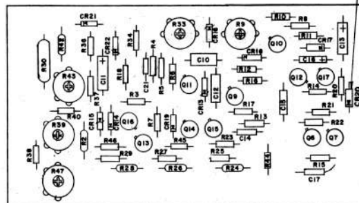
P.C. AMPLIFIER BOARD ASSEMBLY PS-6050-17
