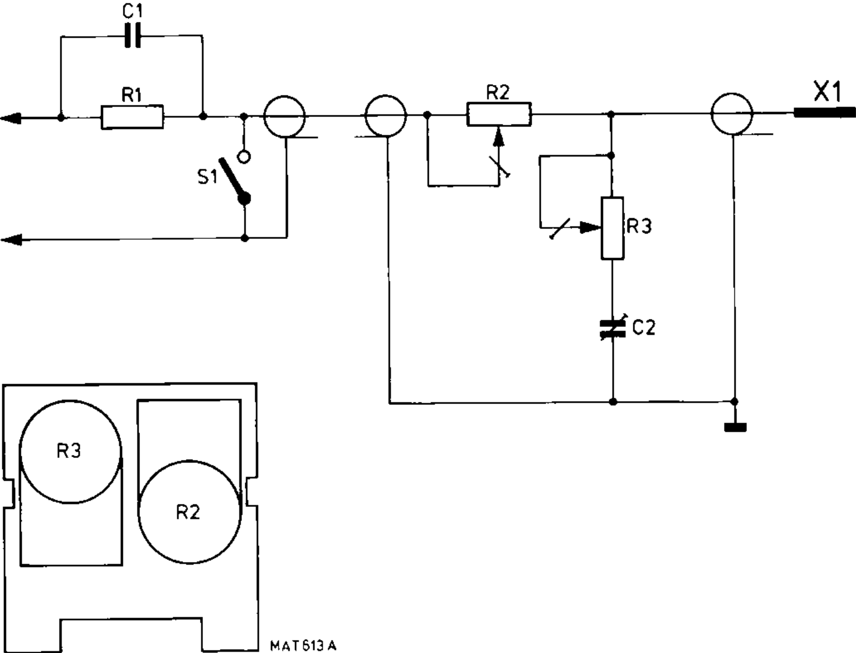
Fig. 12. Printed-wiring board showing adjusting elements, circuit diagram
