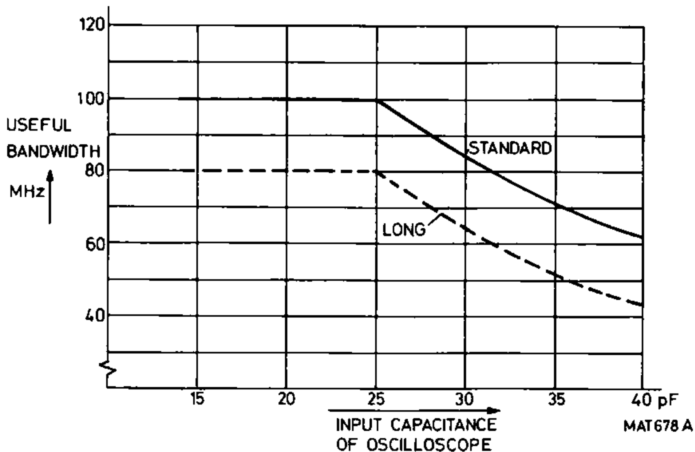
Fig. 3. Useful bandwidth versus input capacitance of oscilloscope
