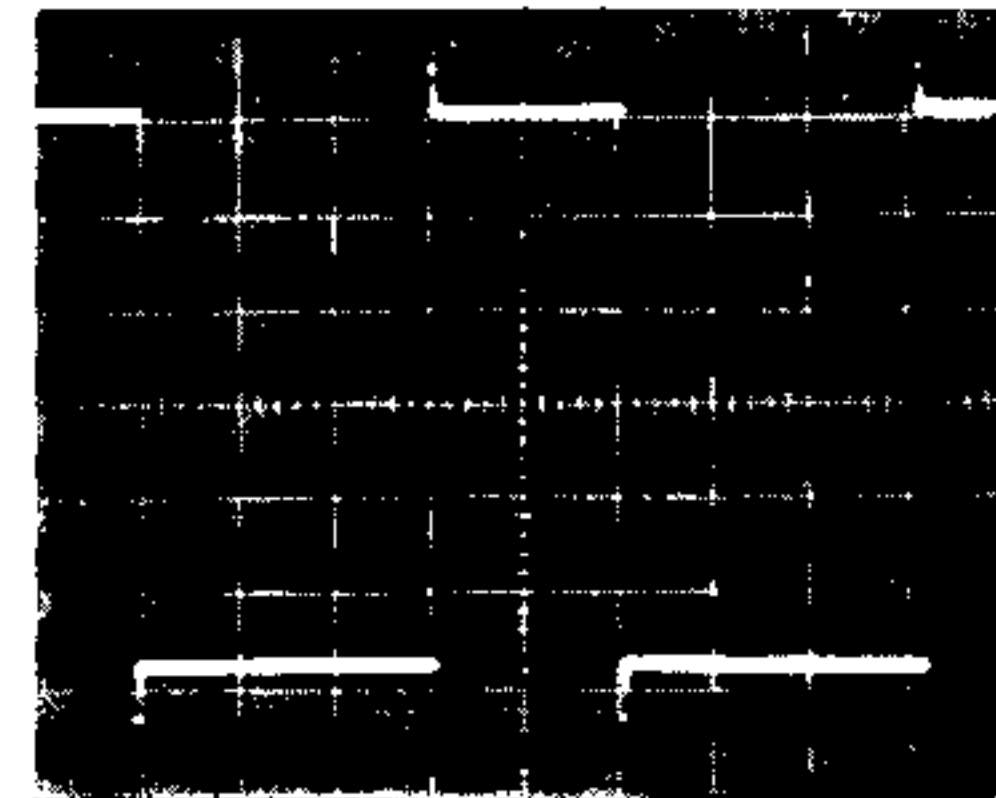
Fig. 9. Overshoot due to incorrectly adjusted potentiometers
