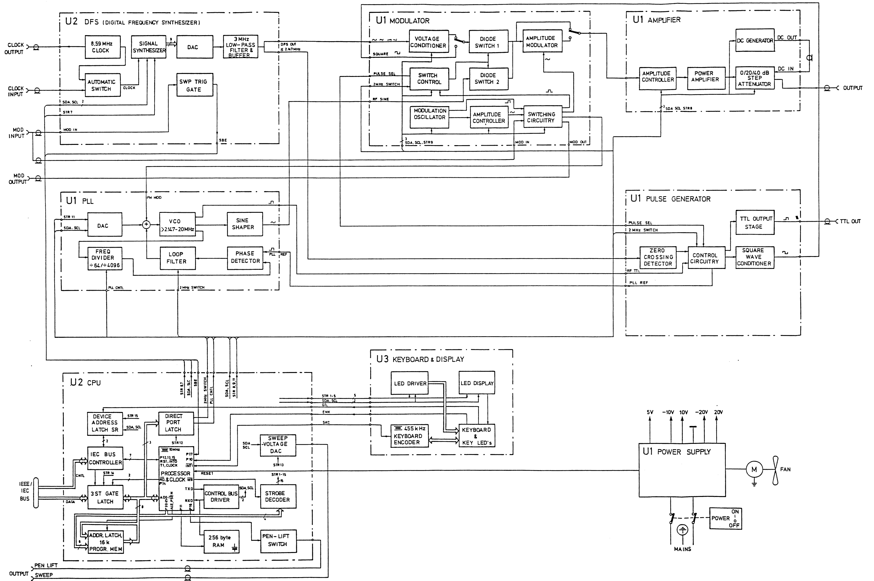
Fig. 30 Block diagram
