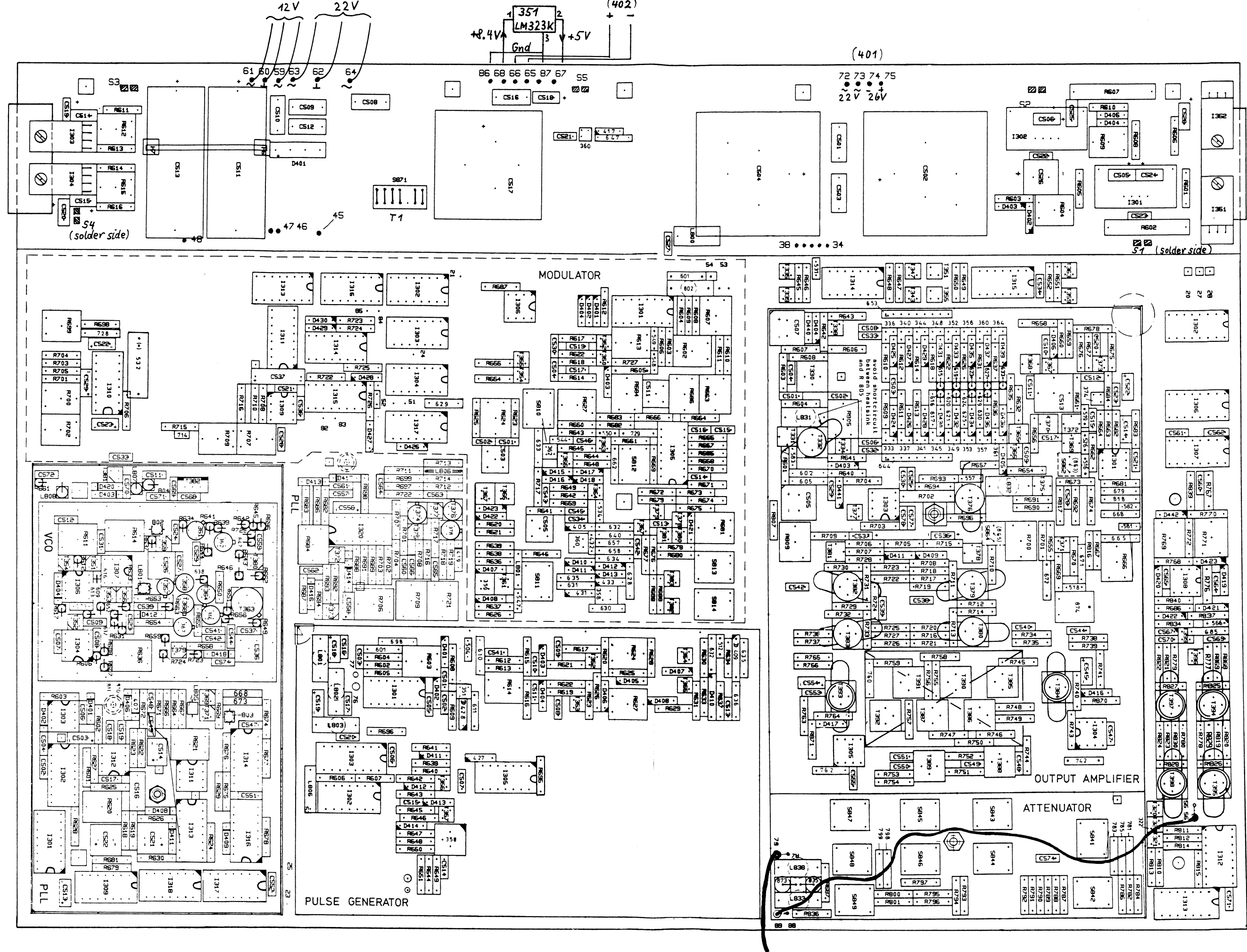
Fig. 34 Unit 1, component lay-out
