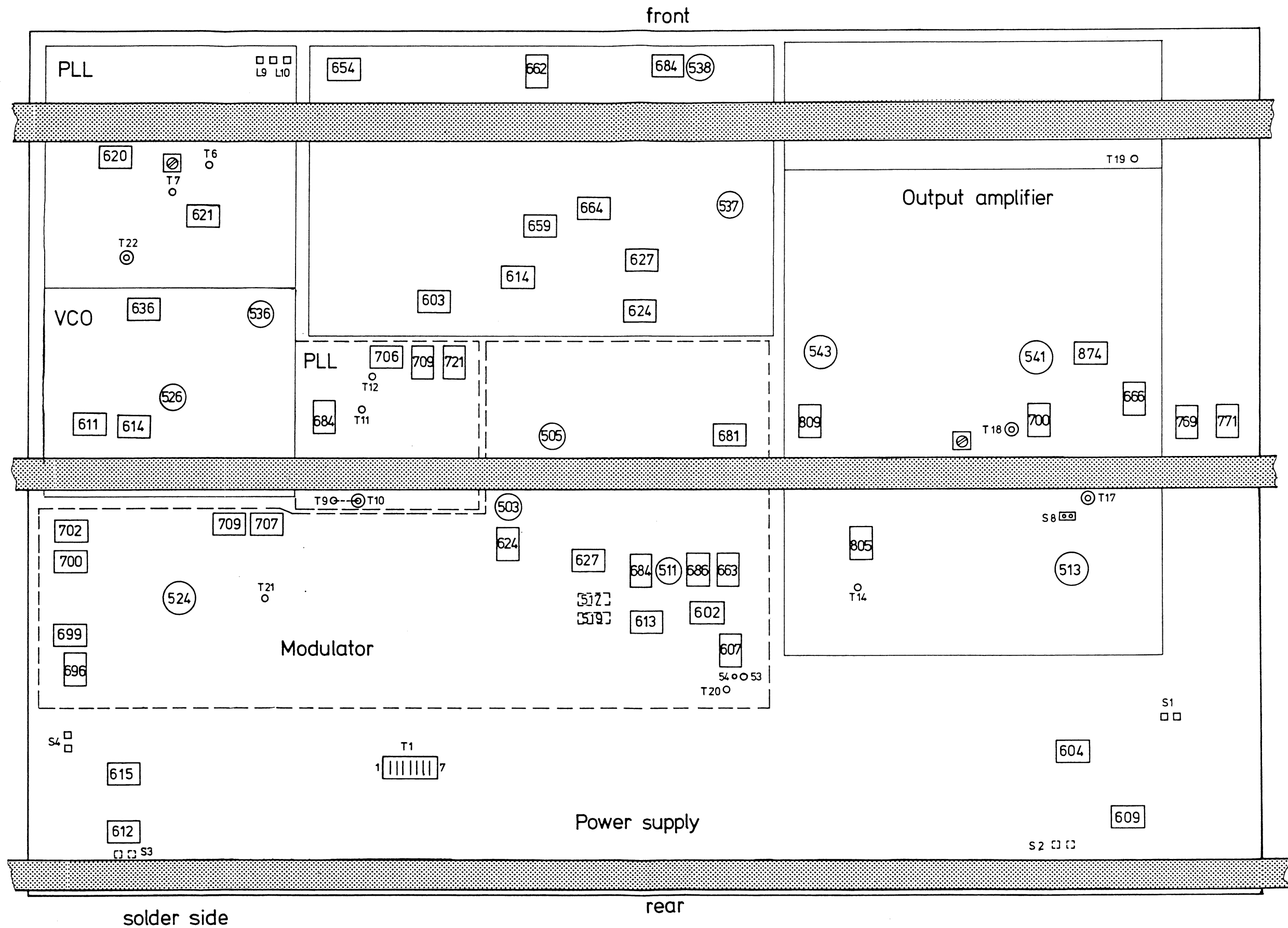
Fig. 29 Unit 1 adjusting elements
