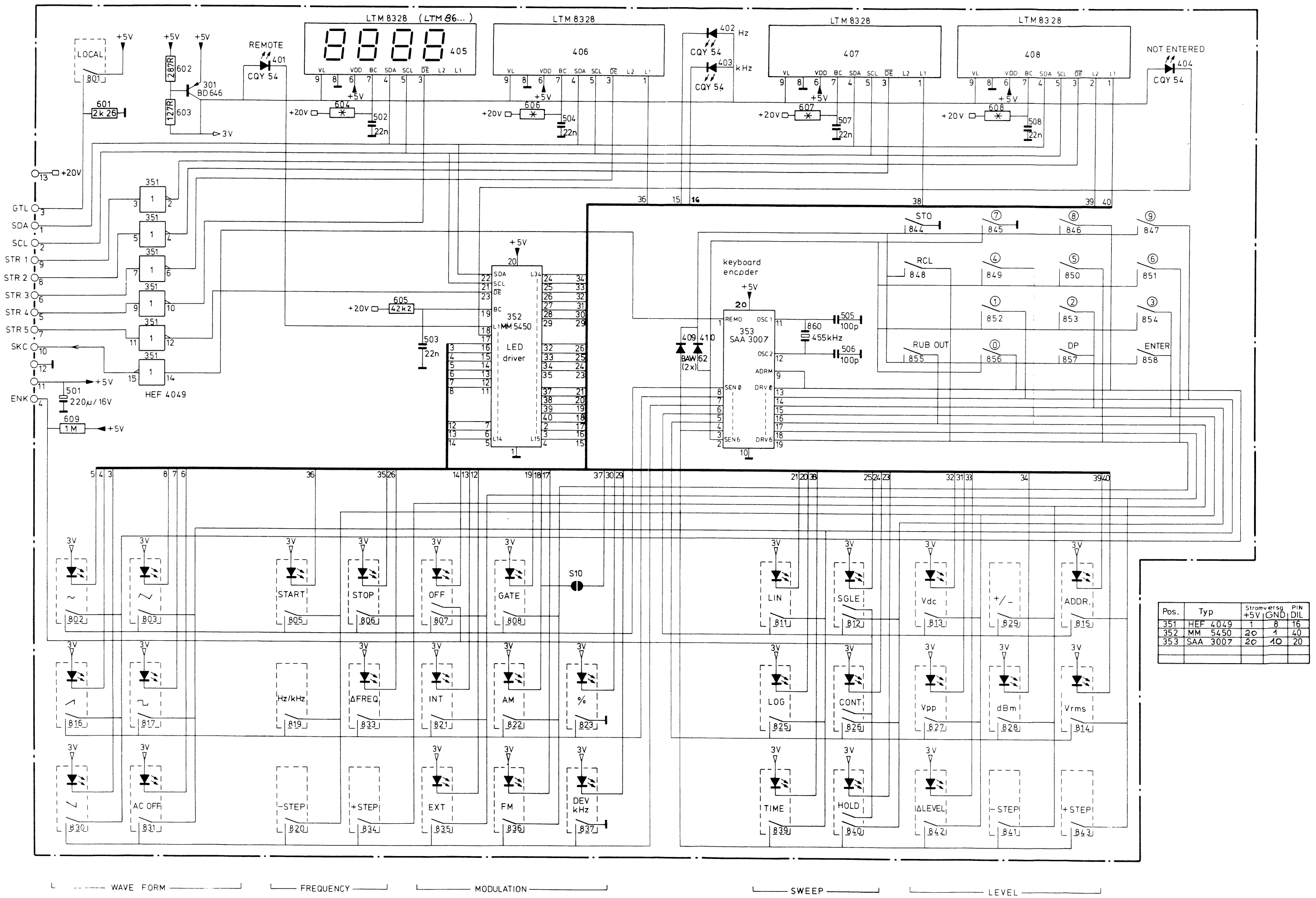
Fig. 43 Unit 3, keyboard display
