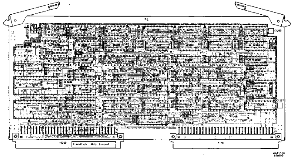
Figure 8.9.1 Unit A9 - DPU UNIT - p.c.b. lay-out.
