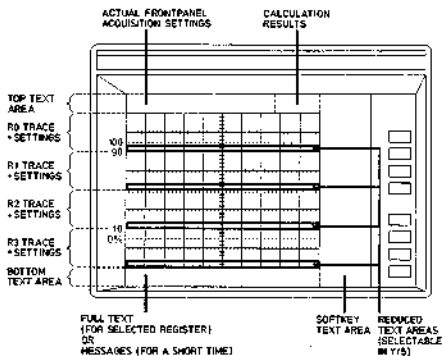
Figure 8.3.1 Screen lay out.
