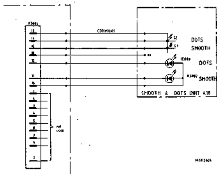
Figure 8.18.2 Unit A18 - SMOOTH + DOTS UNIT - circuit diagram.
