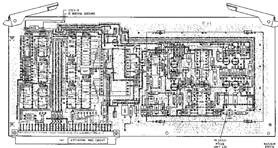
Figure 8.11.2 Unit All - ADC + T&R UNIT - p.c.b. lay-out.
