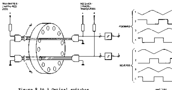
Figure 8.14.1 Optical switches
