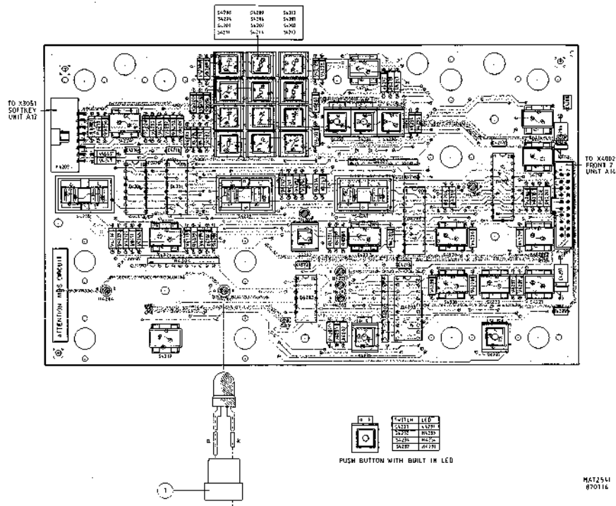
Figure 8.13.1 Unit A13 - FRONT 1 - p.c.b. lay-out.
