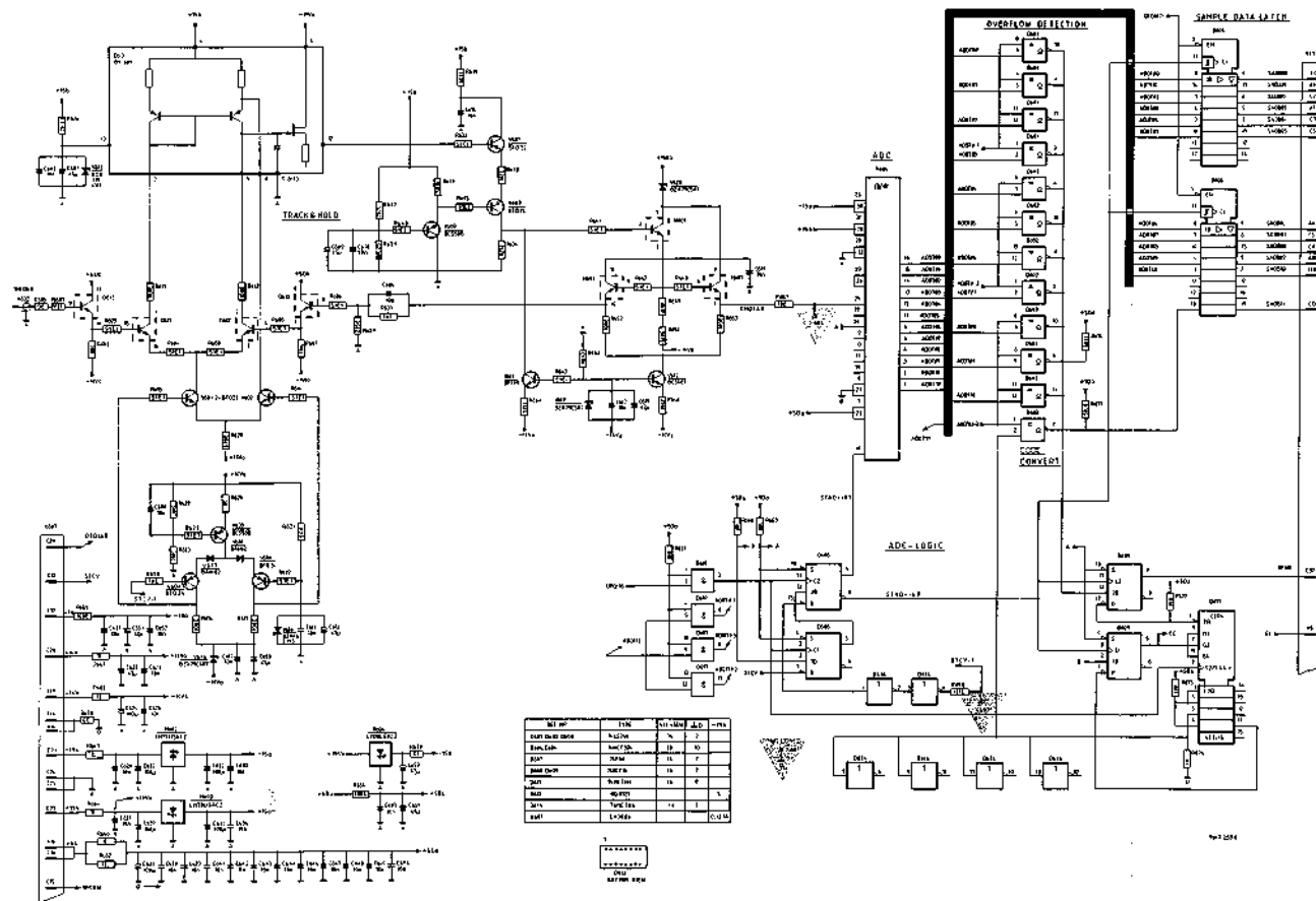
Figure 8.11.3 Unit A11 - ADC + T&amp;H UNIT - circuit diagram.
