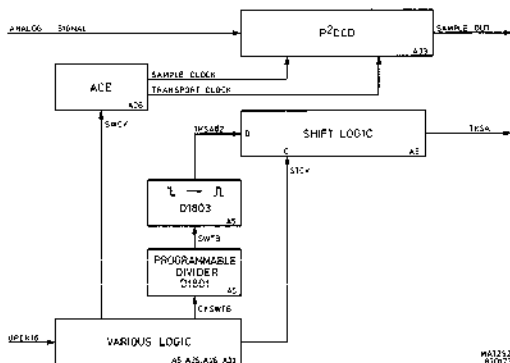
Figure 8.5.1 SHIFT LOGIC
