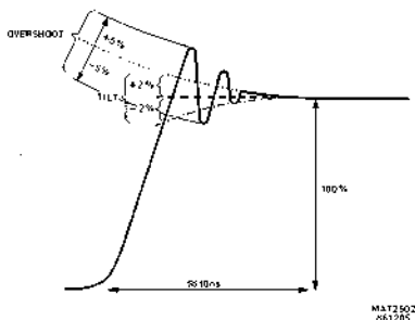
Figure 9.5 HF-pulse response.
