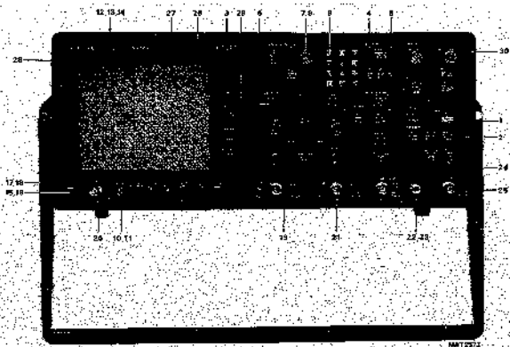
Figure 5-1 Mechanical parts front side
