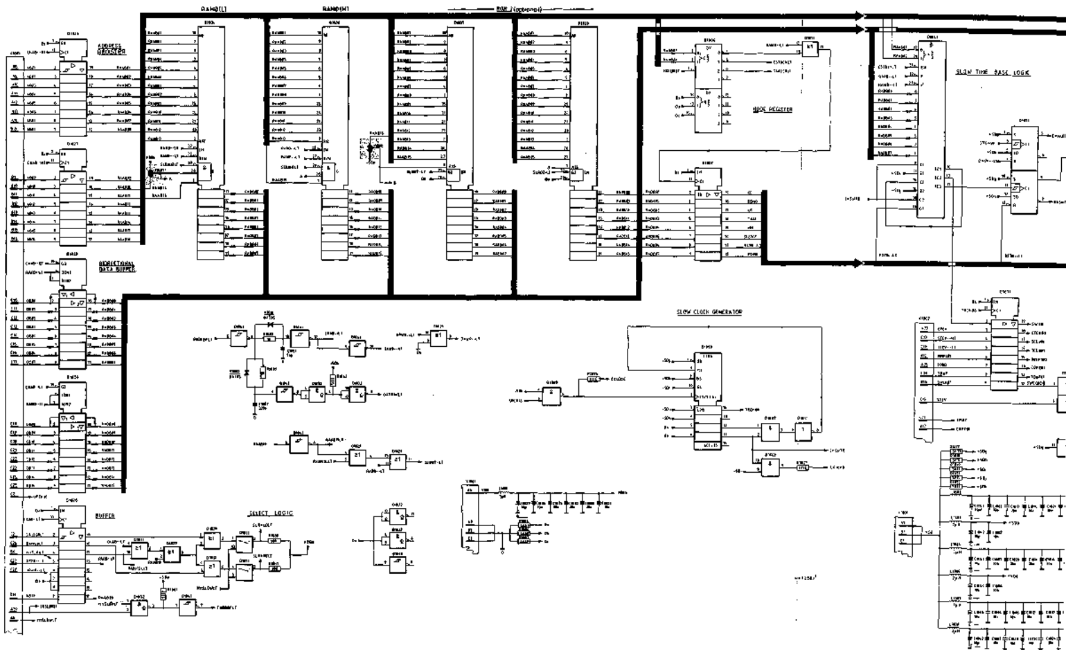
Figure 8.5.3 Unit A5 - MXAM UNIT - circuit diagram.
