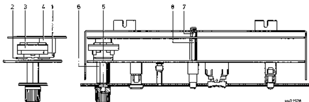
Figure 15.6 Mechanical parts front unit.
