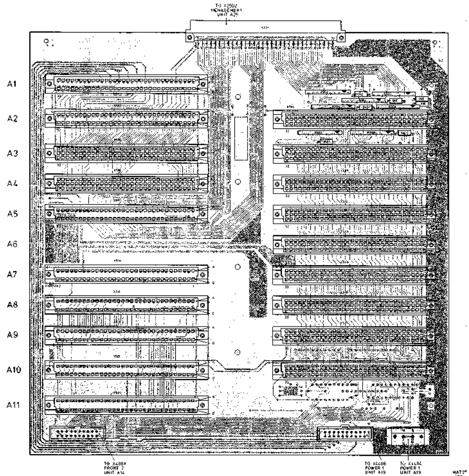
Figure 8.12.2 Unit A12 - MOTHERBOARD - p.c.b. lay-out.
