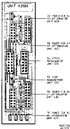
Figure B.35.1 Unit A35 - ATTENUATOR ADAPTION - p.c.b. lay-out.
