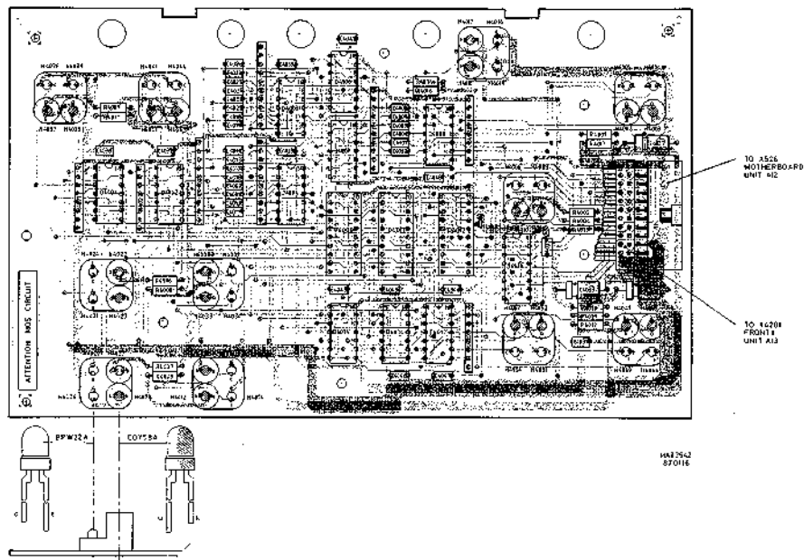
Figure 8.14.2 Unit AI4 - FRONT 2 - p.c.b. lay out.
