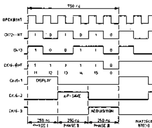
Figure 8.3.6 Clock signals.
