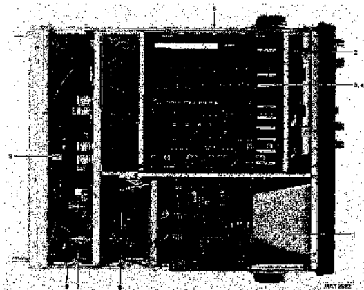
Figure 15.10 Miscellaneous parts.
