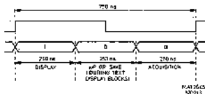
Figure 8.3.3 Display timing.
