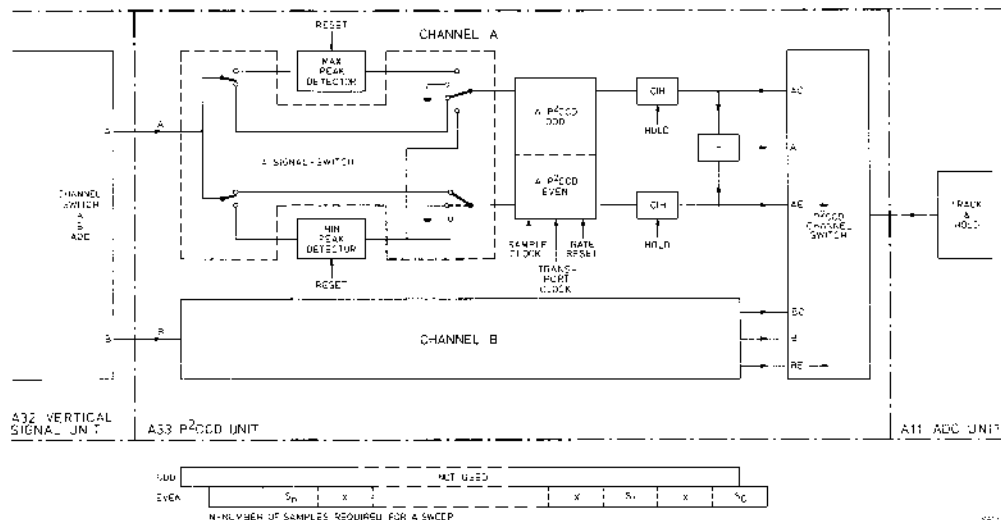
Figure 8.33.11 RANDOM SAMPLING mode Single + Dual channel.
