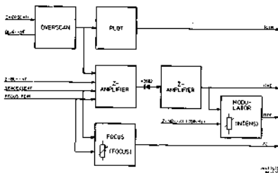
Figure 8.1.4 Blockdiagram 2-circuit.
