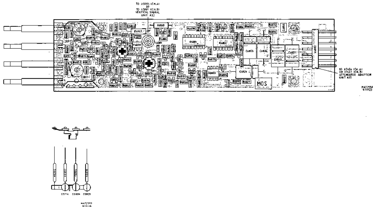
Figure 8.27.1 Unit A27(A29) - HF ATTENUATOR - p.c.b. lay-out.
