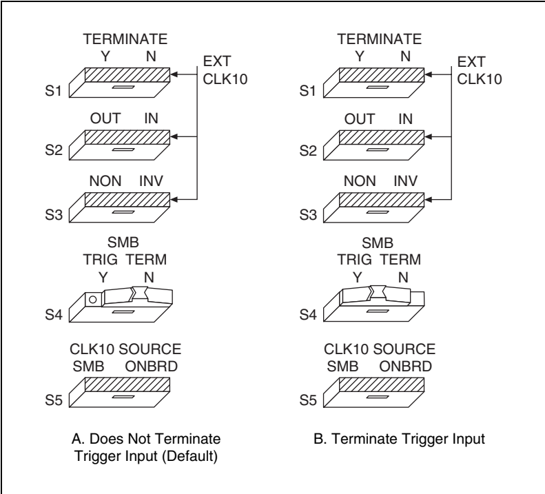
Figure C-9. SMB Trigger Input Termination
