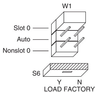
B. Manual Slot 0 Configuration
