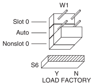
C. Manual Non-Slot 0 Configuration
