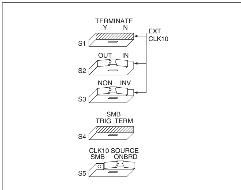
Figure C-8. Drive Noninverted External CLK SMB
