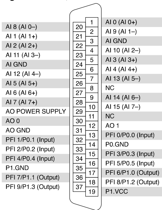
Figure 7. NI PCI/PXI-6233 Pinout
