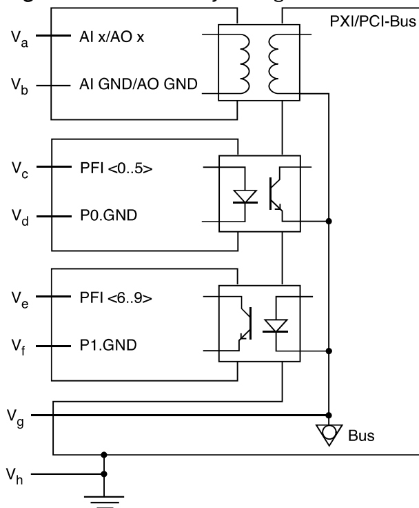
Figure 6. NI 6233 Safety Voltages
