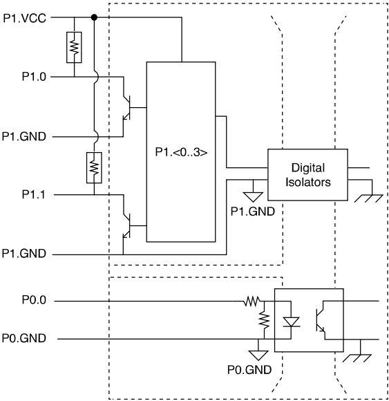
Figure 1. NI 6233 Digital I/O Connections
