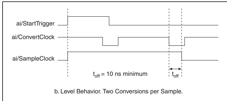
Figure 2-26. ai/SampleClock Output
