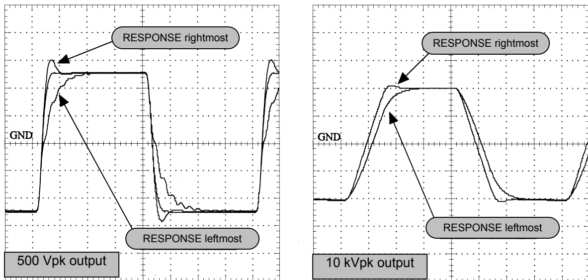
Figure5-6. Step response in constant voltage mode without load
