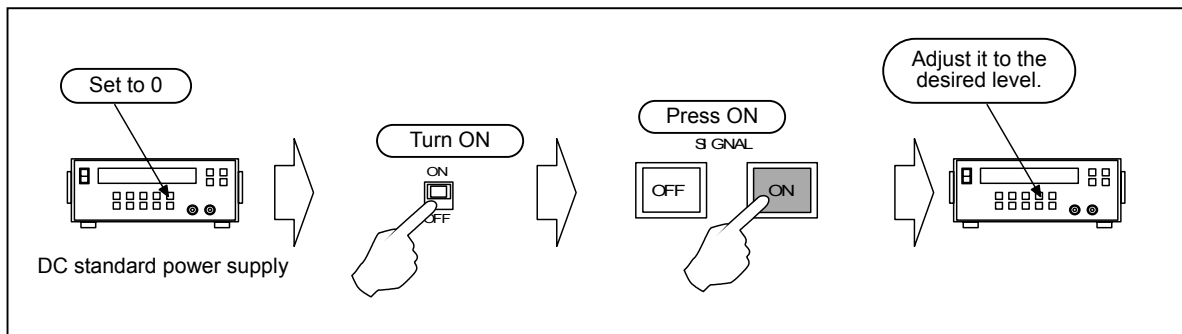
Figure4-33. Using external DC bias signal
