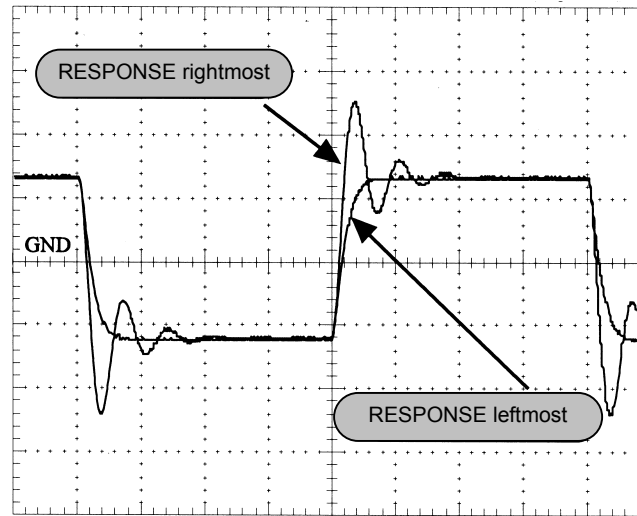
Figure5-10. Step response in constant current mode with 1 M \Omega load
