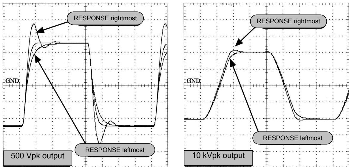
Figure5-7. Step response in constant voltage mode with 35 pF load
