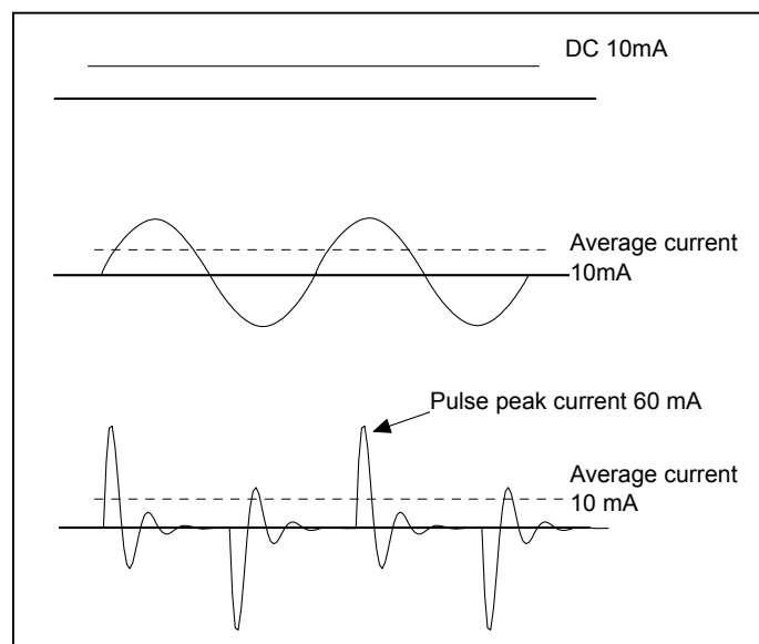
Figure8-1. Output current
