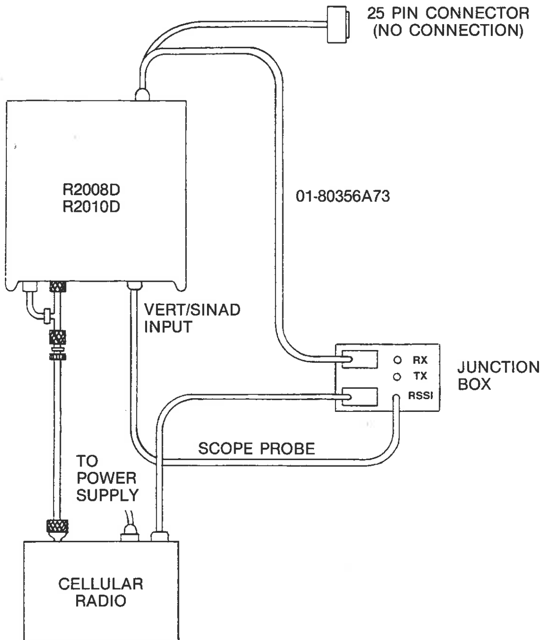
RSSI TESTING
