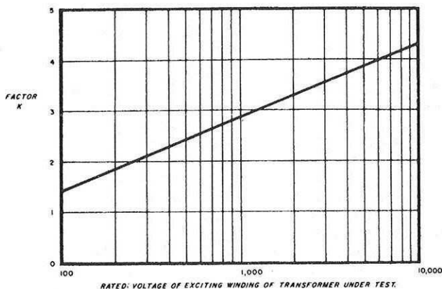
Figure 4 — Approximate values of K for use in correcting TTR readings.
