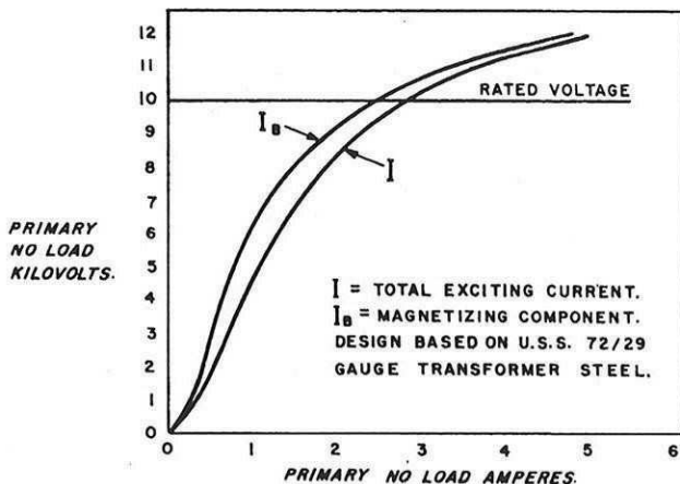
Figure 6: A Transformer magnetizing characteristic.
