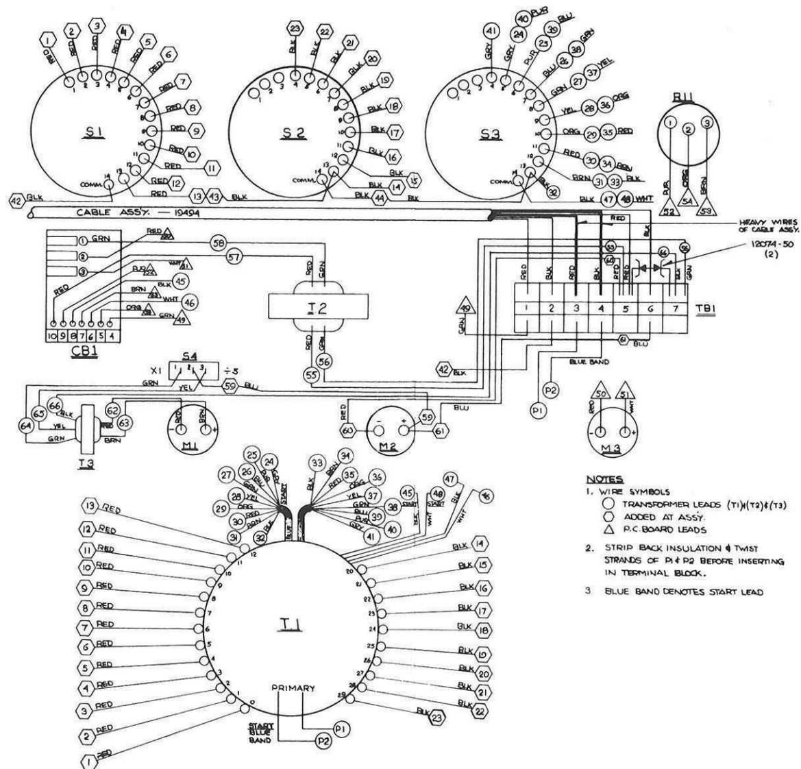
Figure 11: Wiring Diagram of Catalog No. 550005 TTR Set.
