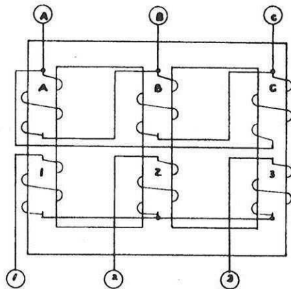
FIGURE 1: Representative Delta-Star Transformer Coil Connections.
