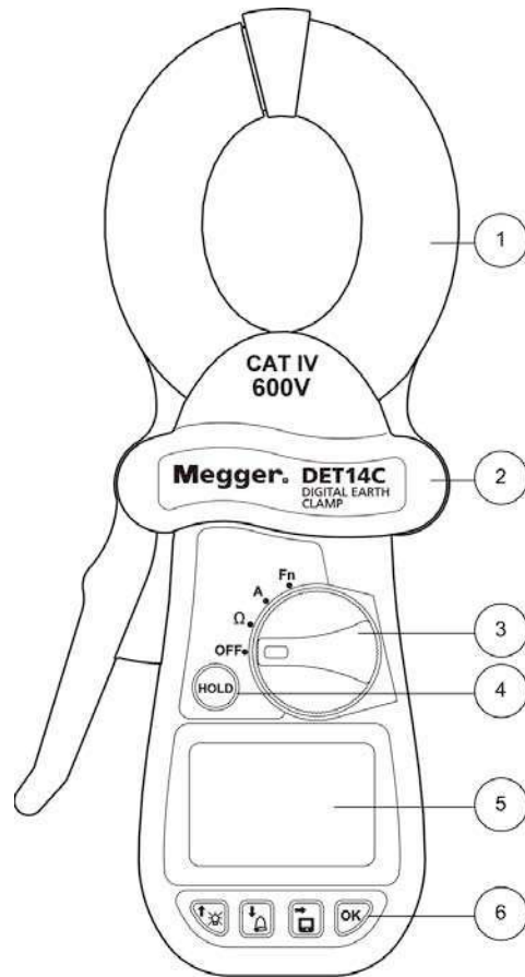
Figure 1: DET14C / DET24C Instrument Front View
