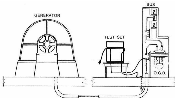
Figure 8: Generator Test Setup.
