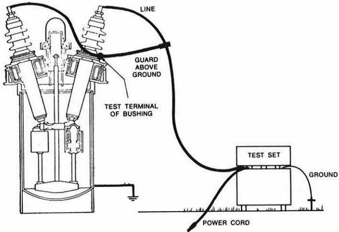
Figure 12: Typical Guard Connection for an Oil Circuit Breaker.
