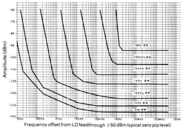
Figure 4: Typical sensitivity vs input frequency.
