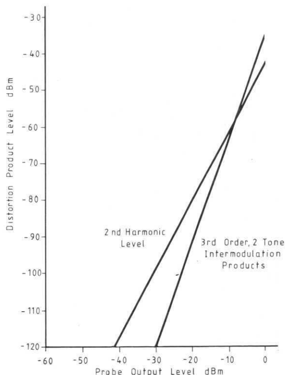
Typical harmonic distortion and intermodulation performance
