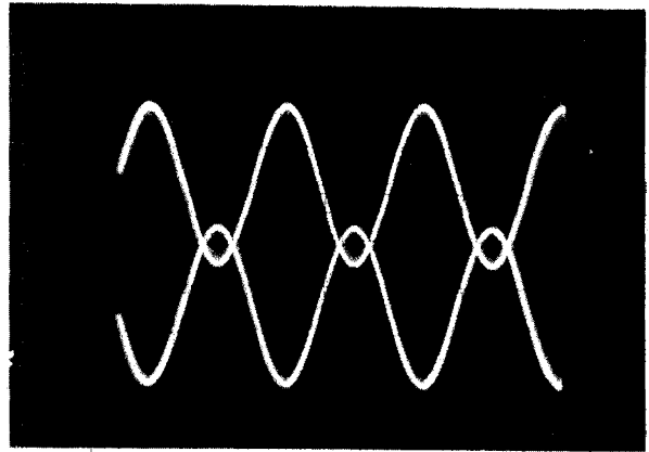
OVER 100% MODULATION
