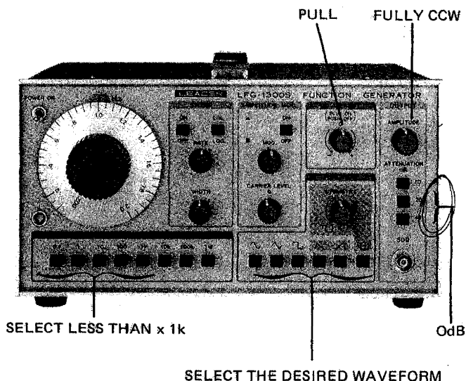
Figure 5-7. DC Offset Operation
