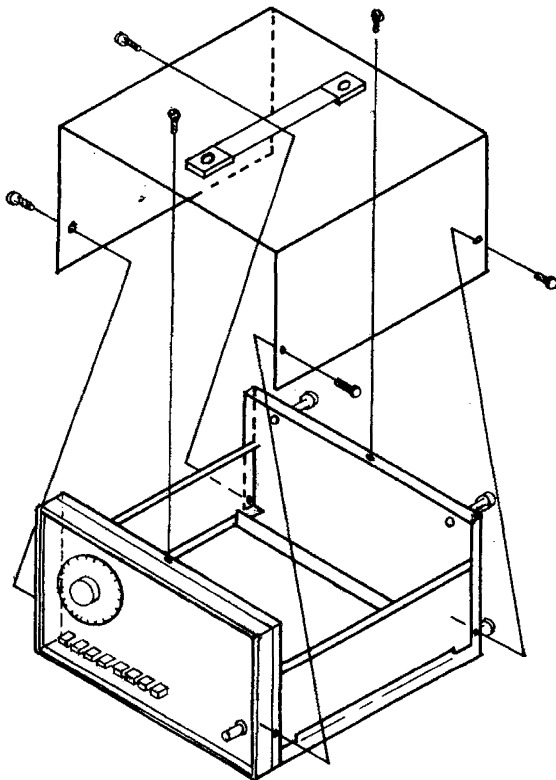
Figure 6-1. Disassembly
