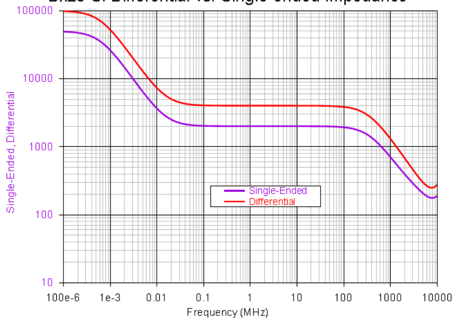
Figure 7-14. Dx20-SI Impedance Graph
