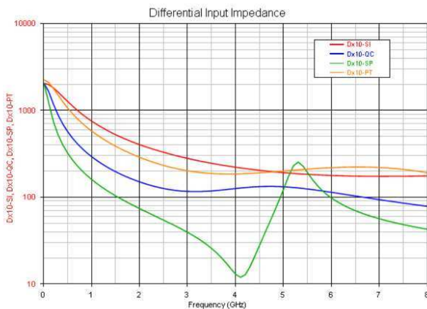
Figure 7-5. Dx10 SI/QC/SP/PT Input Impedance
