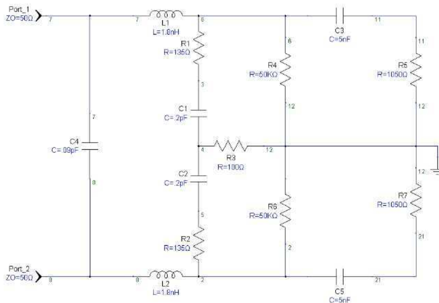
Figure 7-6. Dx10-SI Equivalent Input Circuit
