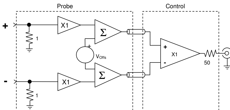
Figure 2. AP034 Block Diagram
