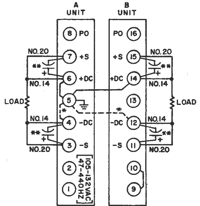
* FOR NEGATIVE GROUND DISCONNECT JUMPERS FROM TERMINALS 5-6, 5-14 AND RECONNECT TO TERMINALS 5-4, 5-12.
