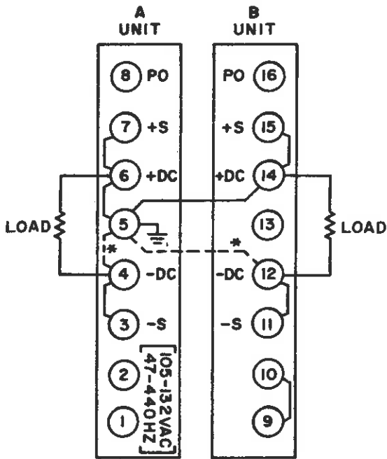
* FOR NEGATIVE GROUND DISCONNECT JUMPERS FROM TERMINALS 5-6, 5-14 AND RECONNECT TO TERMINALS 5-4, 5-12.
