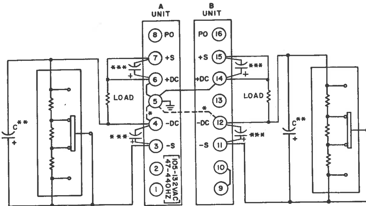
(B) REMOTE SENSING
