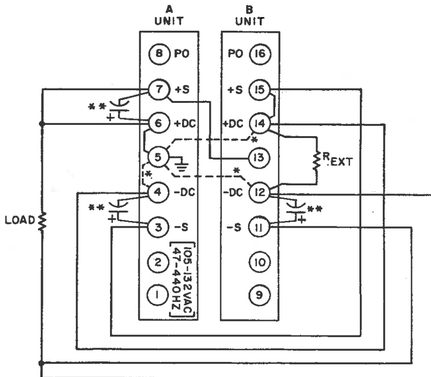
(B) REMOTE SENSING
