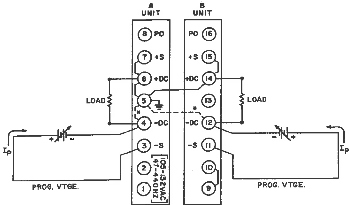
NOTE: OUTPUT VOLTAGE CONTROLS MUST BE SET TO ZERO (A) LOCAL SENSING
