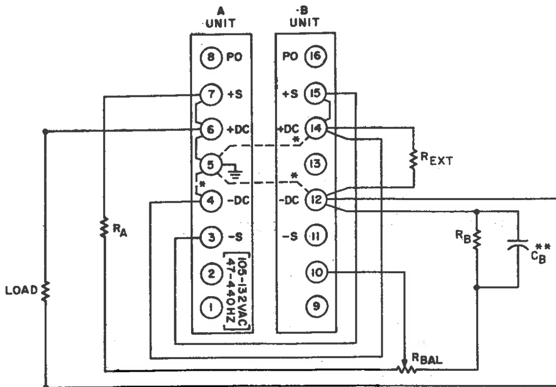
(A) LOCAL SENSING
