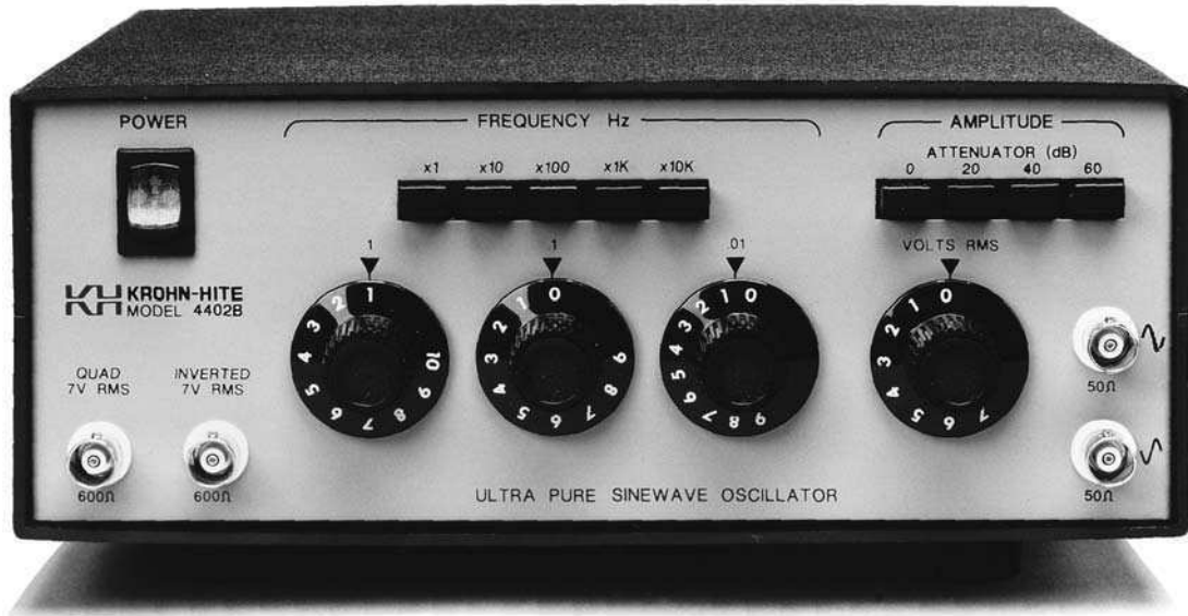
Model 4402B Sinewave Oscillator
