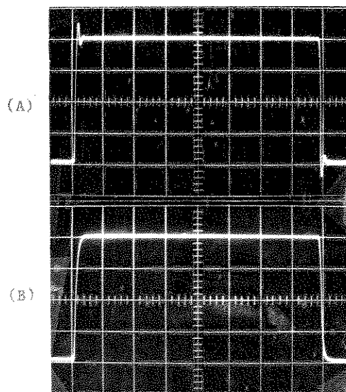
Figure 3. Response to 10kHz Square Wave with Cutoffs at 10Hz and 1MHz. (A) Butterworth (B) RC
