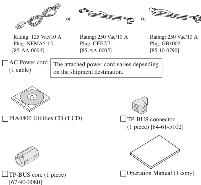
Fig. 1-2 Accessories
