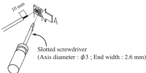
Fig. 2-4 Connection to the SHUT DOWN connector
