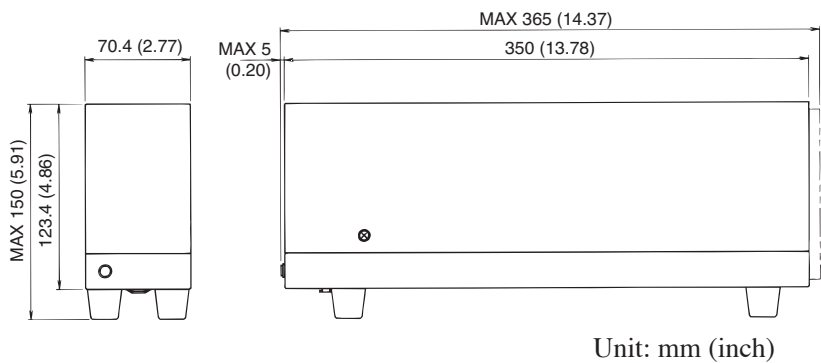
Fig. 5-1 External dimensions
