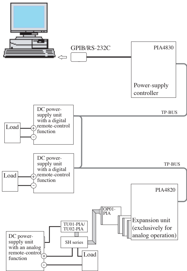
Fig. 1 System Configuration
