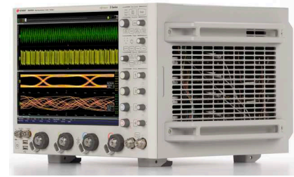
The Infiniium Z-Series captures rise times as fast as 5 ps (20/80).
