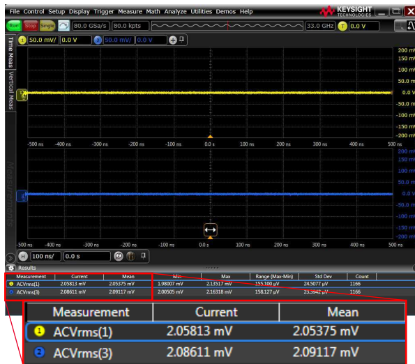
Ultra-low noise at 33-GHz full bandwidth (2.10 mV at 50 mV/div).
