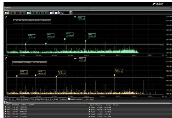
Improved calibration increases the spurious free dynamic range by up to 15 dBc.
