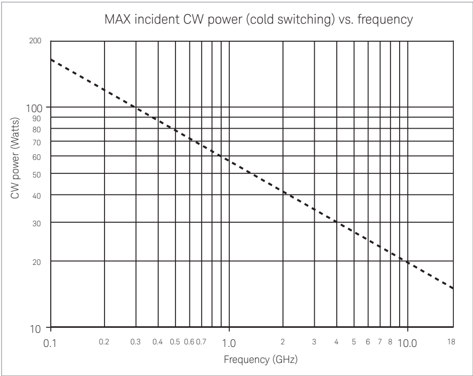
Figure 6. Maximum incident CW power across frequency
