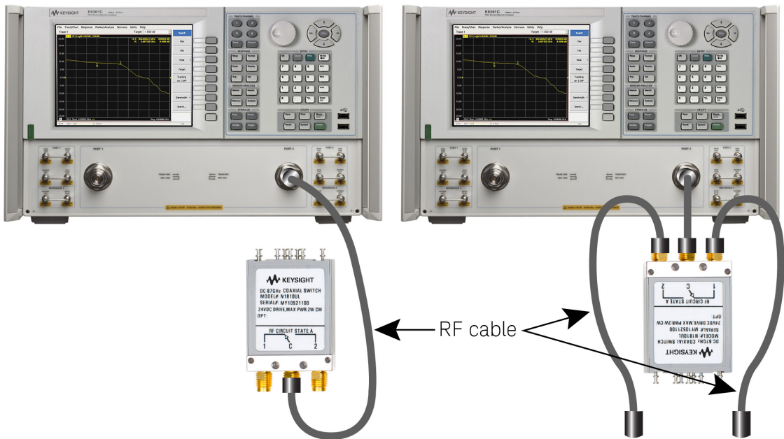
Figure 1. How a conventional switch is connected to a measuring instrument
